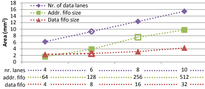
Figure 7.10: R-GPU area costs of the communication network (4 to 10 lanes), address FIFOs (64 to 512 entries) and data FIFOs (4 to 32 entries).
