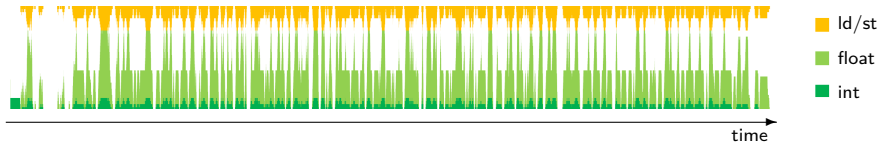
Figure 7.9: Activity of the cores within one SM in R-GPU over the execution of the 2D-convolution application. The activity is split into integer (int), floating point (float) and load-store (ld/st) operations.
