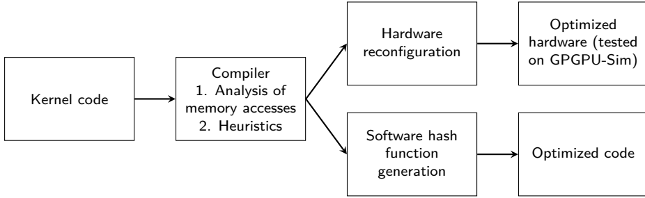
Figure 6.7: Our framework for bank conflict reduction. It encompasses hardware and software approaches.
