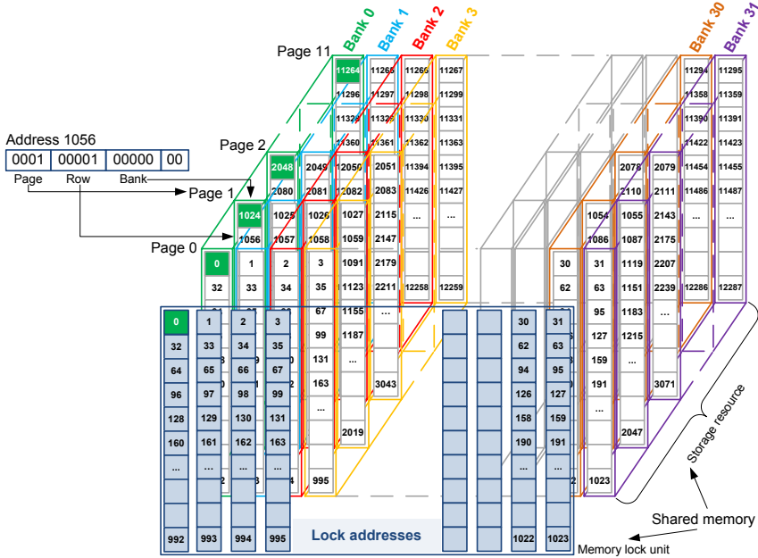
Figure 2.6: Scratchpad memory layout on an NVIDIA Fermi GPU. The 48 kB of memory is accessed via 4-byte words and is distributed over 32 banks. Each bank has 32 lock bits available for atomic operations. [105]
