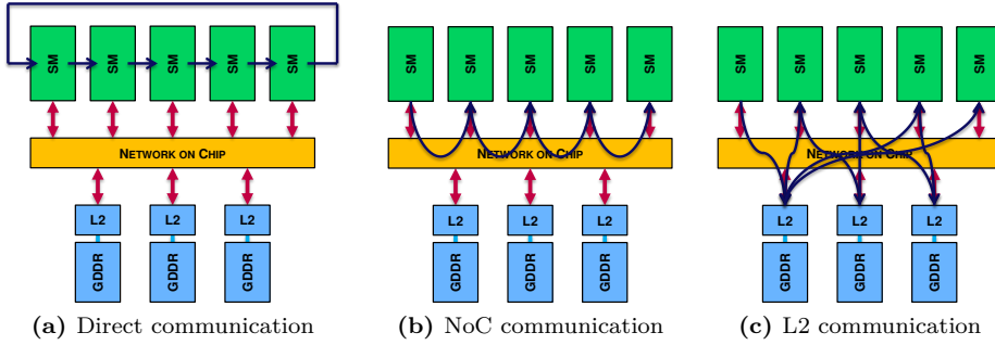
Figure 7.3: Three options for inter SM communication.
