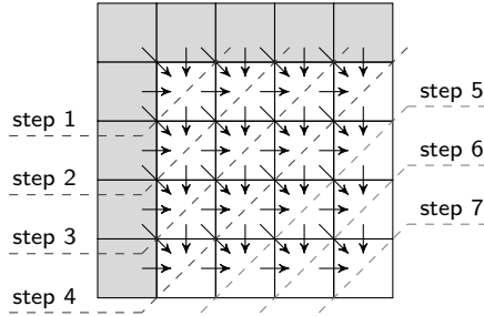
Figure 7.8: Dependencies between matrix elements in the Needleman-Wunsch algorithm. Seven steps are required to calculate this 4 \times 4 matrix.
