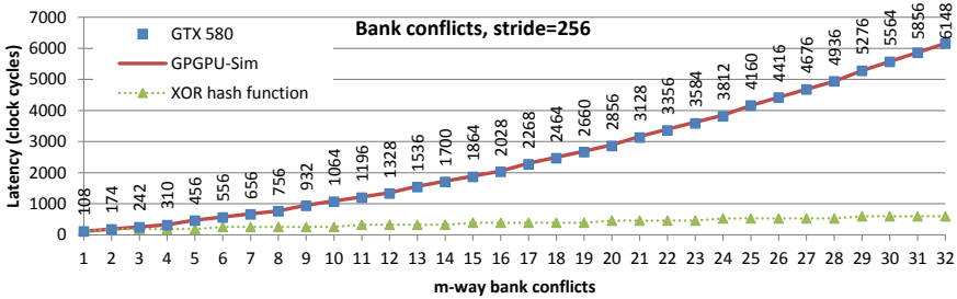
(c) m -way intra-warp bank conflicts in the simulator, m is given by the number of threads accessing different addresses in the same bank, but an extra lock conflicts appears every four bank conflicts
