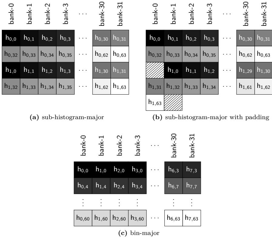
Figure 3.3: Three different methods of placing eight sub-histograms of a 64-bin histogram in a banked memory. Each bin in a sub-histogram is labeled h_{s,b} where s is the sub-histogram number and b is the bin index. In (a) and (b) the first two sub-histograms are shown, placed in a sub-histogram-major order. In (c) a part of the bins 0, 3, 4, 7, 60 and 63 for the eight sub-histograms is shown, placed in a bin-major order.
