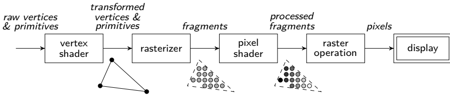
Figure 1.1: Basic graphics rendering pipeline. At the left primitives and vertices forming a 3D scene enter the pipeline. A primitive consists of one or more vertices. Each vertex has attributes such as position, color and texture. The vertex shader transforms the vertices' coordinates and projects them on the virtual camera's film plane. The rasterizer converts the triangles into fragments and the pixel shader maps a texture to them. Finally all fragments are combined into a 2D array of pixels to be displayed.
