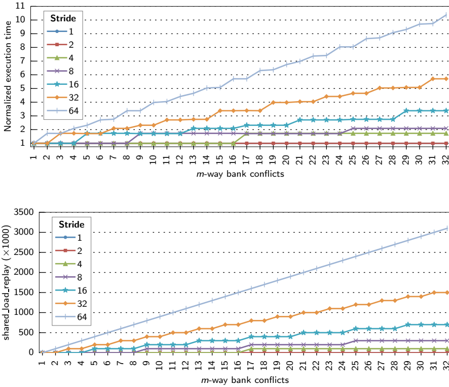
Figure 6.2: Execution results on NVIDIA K20 for access patterns to scratchpad memory with different bank conflict degrees ( m -way) and strides. (Top) Normalized execution time; (Bottom) Profiling results.
