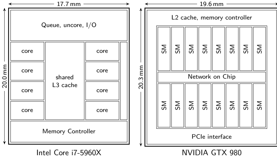
Figure 2.1: Chip layout comparison of an Intel® Core™ i7-5960X eight core CPU and an NVIDIA GTX 980 with sixteen Streaming Multiprocessors (SMs).
