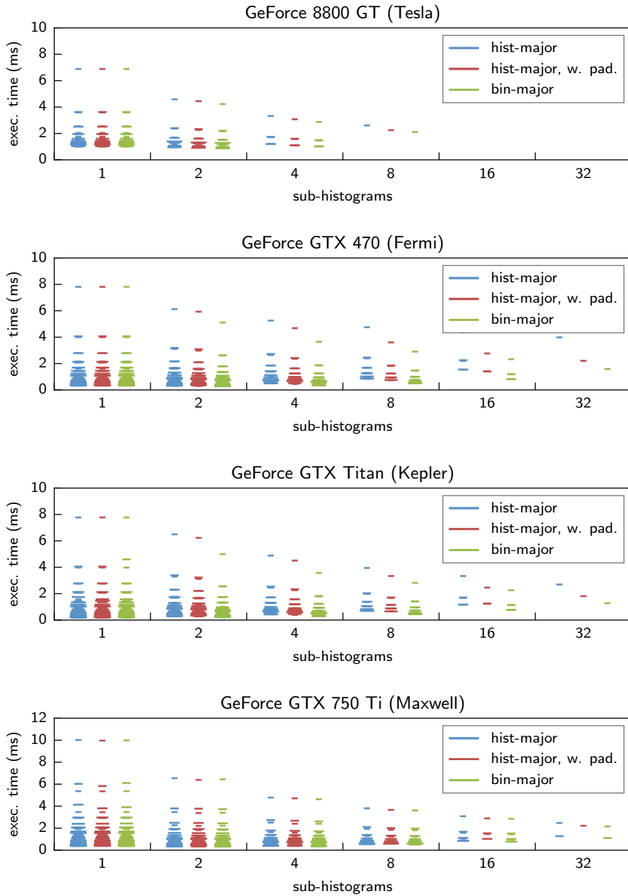
Figure 3.9: 256-bin histogram on four GPUs using a private histogram for each warp
