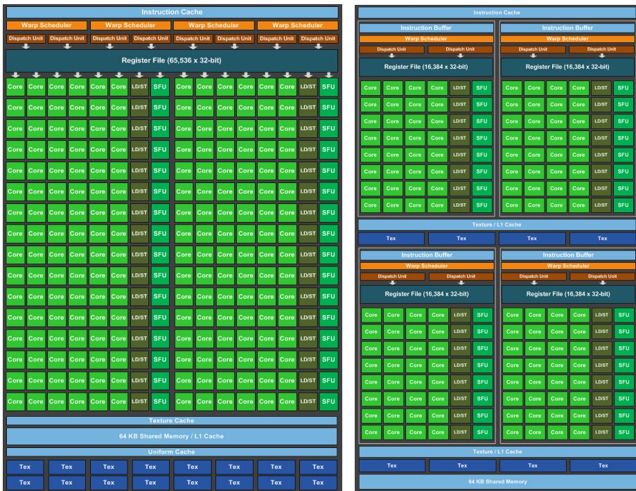
Figure 2.5: Kepler [78] and Maxwell [84] Streaming multiprocessor (SM) design.
