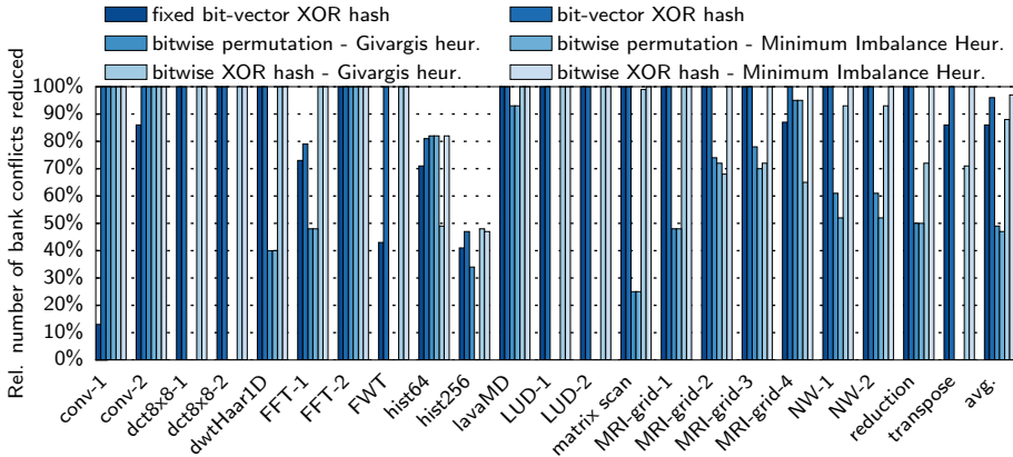
Figure 6.8: Relative number of bank conflicts removed by various hash function compared to a baseline GPU (no hash function) for a set of benchmarks.
