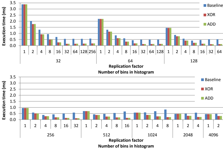
Figure 5.6: Histogram execution time, configured for 32 up to 4096 bins. Replication (sub-histogram-major without padding) is used to improve performance. Results are averaged over 24 12-bit grayscale images [1] of 1536 \times 1024 pixels and are shown for the baseline, XOR and ADD hash function.
