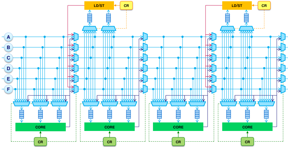
Figure 7.2: Design of the R-GPU architecture. Cores and load-store units communicate via FIFO buffers and six data lanes named A to F . The single instruction each core executes is stored in a local configuration register (CR). Only four of the 32 cores and two of the 16 load-store units in an SM are shown for clarity.
