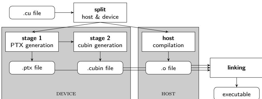
Figure 2.7: CUDA compilation consists of two parts: host and device.
