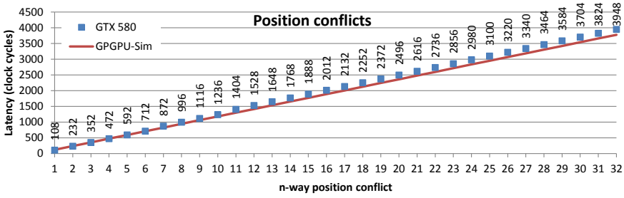
(a) n -way intra-warp position conflicts, in each test, n threads update the same location
