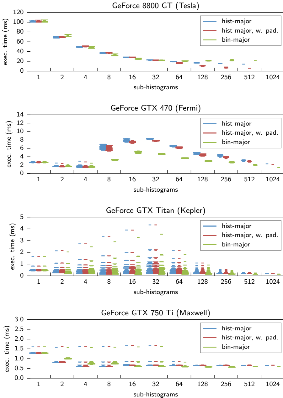
Figure 3.4: 256-bin histogram on four GPUs using atomic operations on global memory
