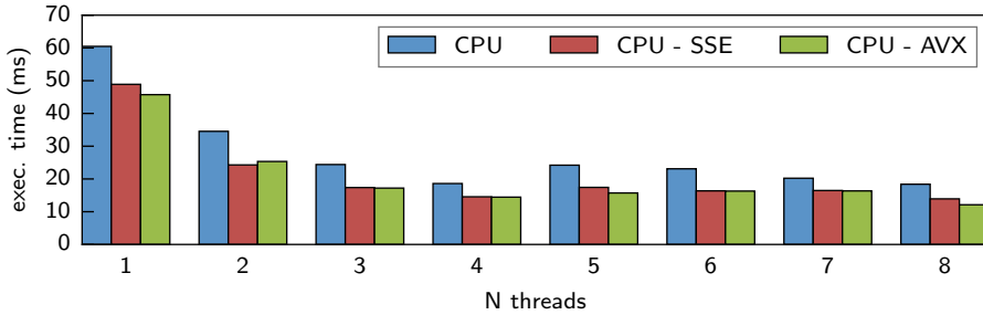
Figure 4.5: Hough transform on a CPU (Intel® Core™ i7-4770) using 1 to 8 threads
