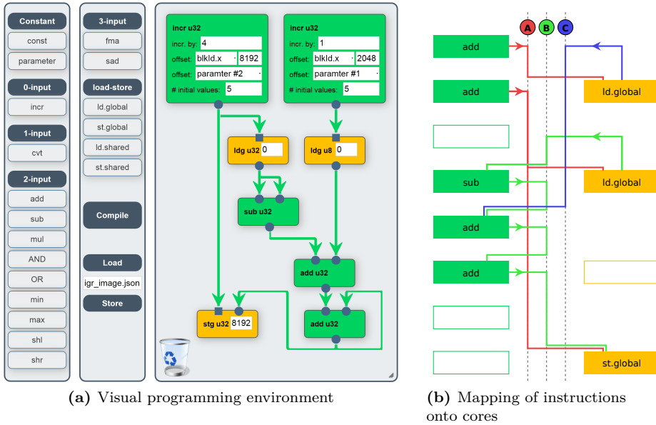
Figure 7.5: Integral image application programmed in the visual programming environment (a) and the resulting mapping to cores and load-store units (b).
