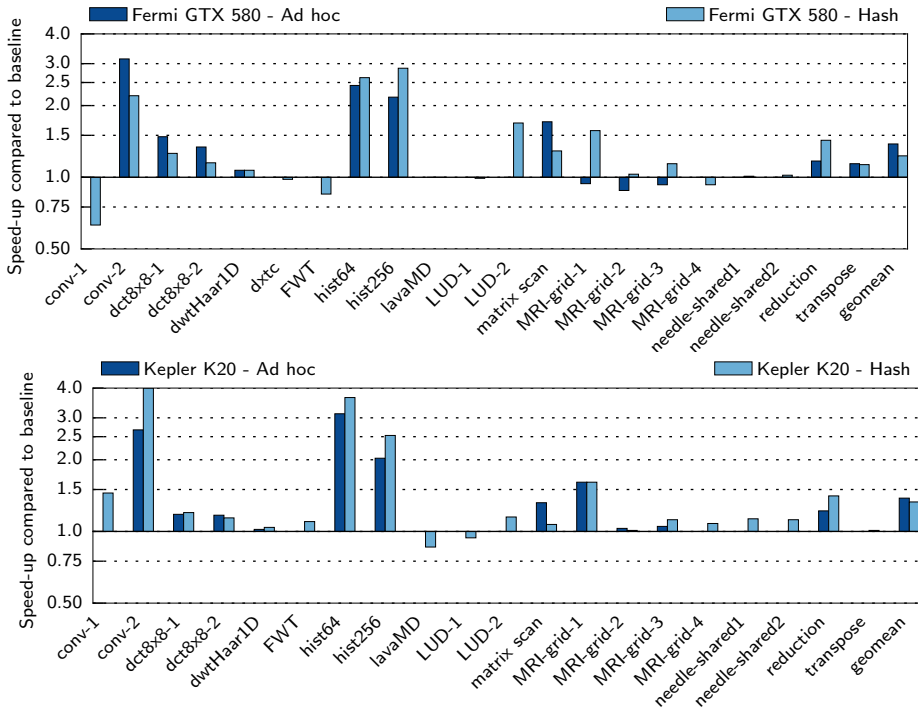
Figure 6.11: Overall speed-up obtained by an ad-hoc optimization technique (typically, padding), and a bit-vector XOR hash function compared to a baseline implementation (neither hash function, nor ad-hoc technique) for a set of benchmarks, on GTX 580 (Fermi) and K20 (Kepler). dxtc has been tested on GTX 280 (Tesla architecture).
