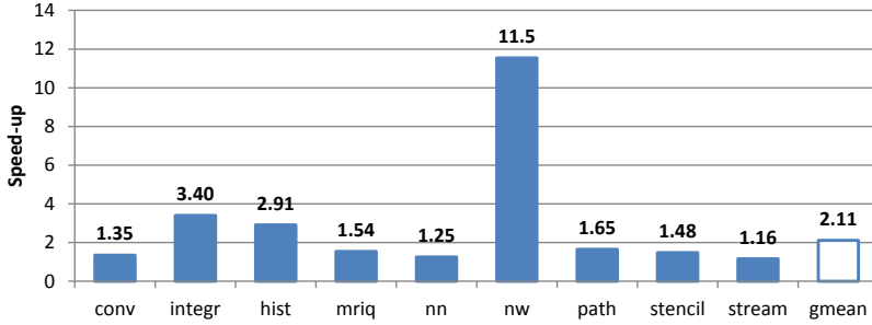
Figure 7.7: Speed-up of R-GPU compared to an optimized GPU implementation
