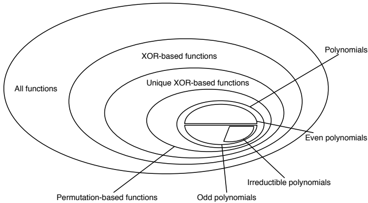
Figure 6.3: Classification of different types of hash functions as given by Vandierendonck and De Bosschere [111]
