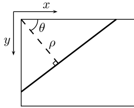
Figure 4.4: Polar representation of a line.
