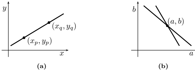
Figure 4.3: (a) A line through two points in an image. (b) Two lines (sets of votes) in the Hough space corresponding to the two points.
