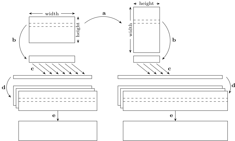
Figure 4.9: Input-data independent implementation of the Hough transform on GPU. First the image is rotated by the first kernel (a). In a second kernel each thread block copies a part of the input image from the global (off-chip) memory to the scratchpad (on-chip) memory (b). Then one Hough line is calculated in scratchpad memory based on the part of the image in the scratchpad memory (c). This line is stored in a sub-Hough space in global memory (d). This step is repeated to calculate the next Hough line, until one entire sub-Hough space is filled by each thread block. A third kernel sums all sub-Hough spaces together to make the final Hough space (e).
