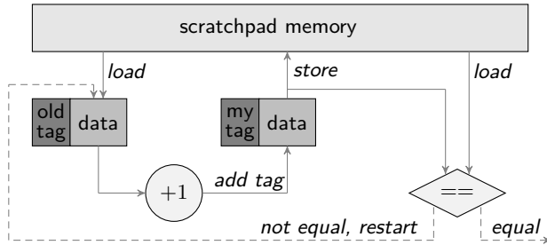
Figure 3.7: Block diagram of the software atomic operations [73].
