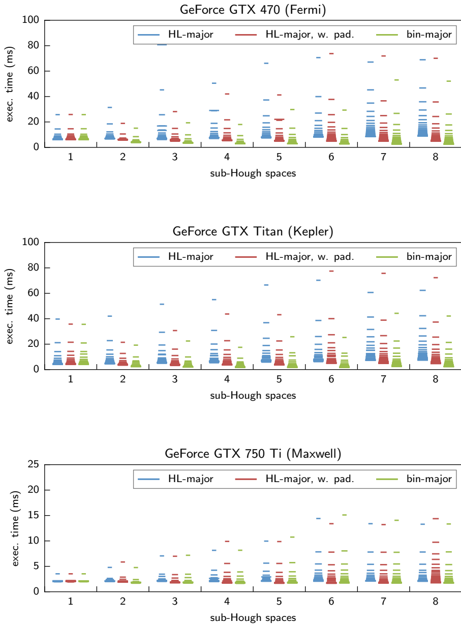
Figure 4.8: Hough transform on GPU using scratchpad memory atomic operations.
