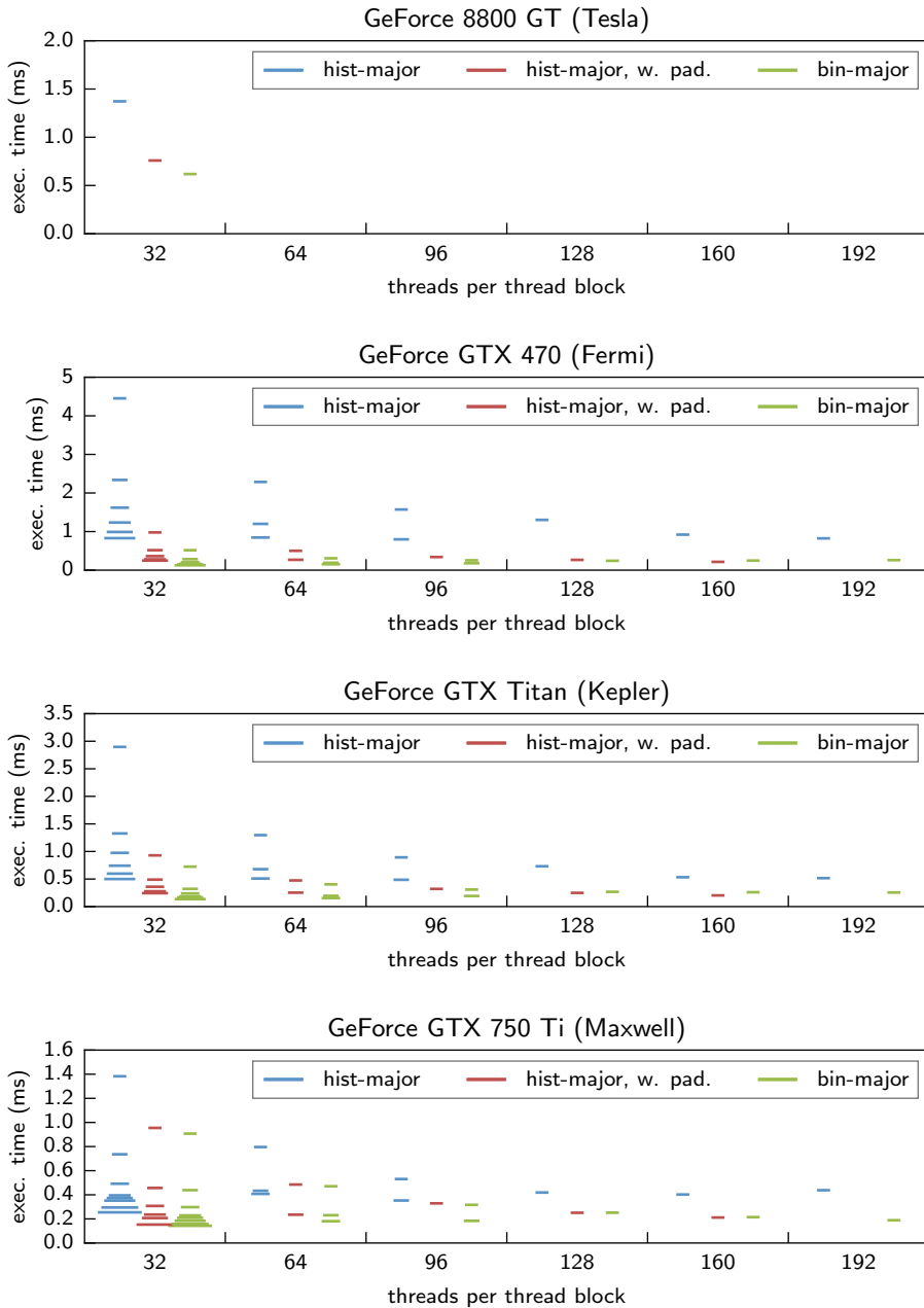
Figure 3.6: 64-bin histogram on four GPUs using a private histogram for each thread
