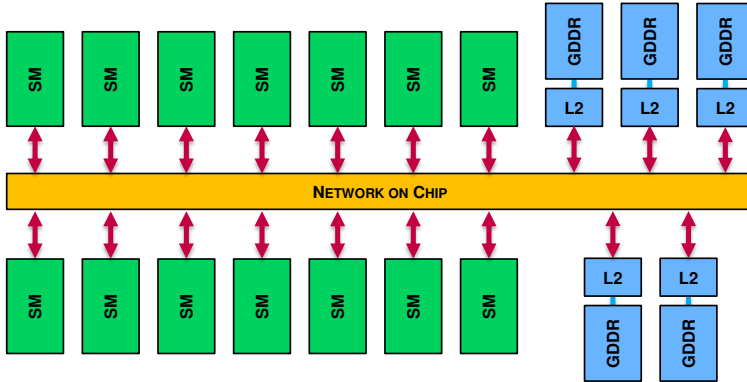
Figure 2.3: A GPU consisting of 14 SMs and 5 memory partitions (GDDR) with L2 cache, all connected by a network on chip. This specific configuration can be found in an NVIDIA GTX 470.
