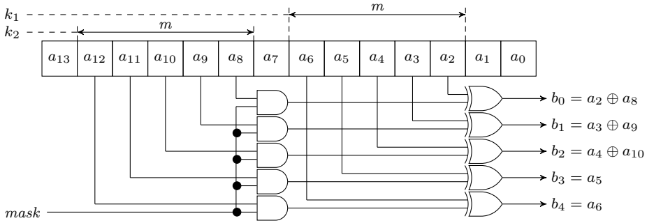
Figure 6.5: The bit-vector exhaustive search algorithm selects the best values for k_1 , k_2 and mask , in this example k_1 = 2 , k_2 = 8 and mask = 7 .
