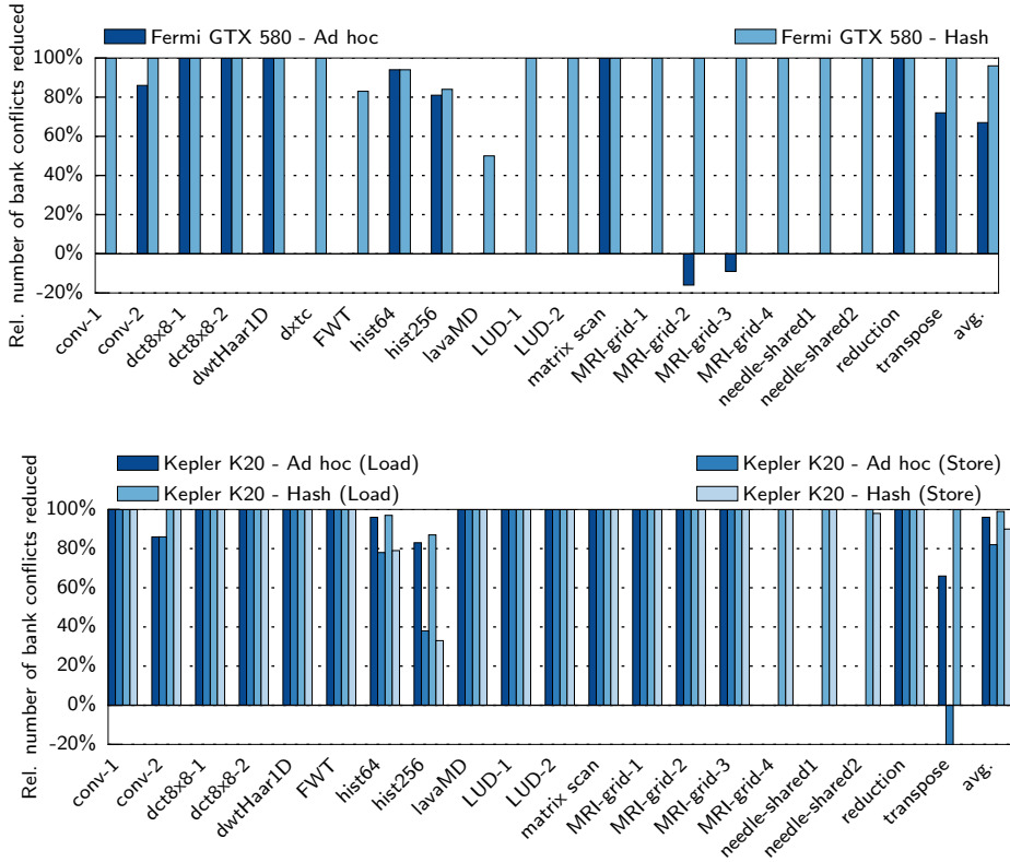
Figure 6.10: Relative number of bank conflicts removed by an ad-hoc optimization technique (typically, padding), and a bit-vector XOR hash function compared to a baseline implementation (neither hash function, nor ad-hoc technique) for a set of benchmarks, on GTX 580 (Fermi) and K20 (Kepler). dxtc has been tested on GTX 280 (Tesla architecture).
