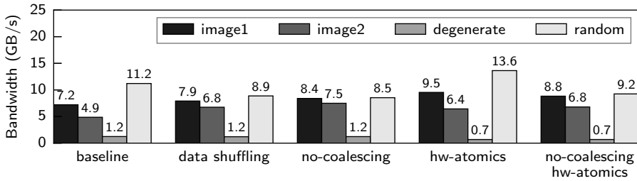
Figure 3.8: Results from [73] (Section 6) for a 256-bin histogram using a private sub-histogram per warp on a GeForce GTX 470. Four extensions to the baseline by Podlozhnyuk in [92] are evaluated for four images.
