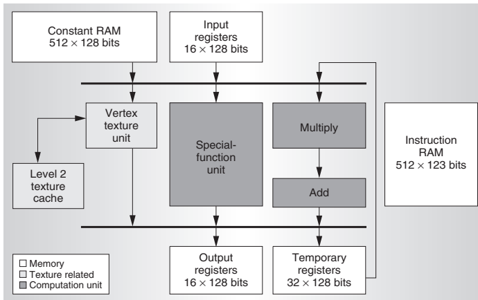
Figure 1.3: GeForce 6800 vertex processor block diagram consisting of a vector multiply-add unit, a scalar special-function unit and a texture unit. [61]
