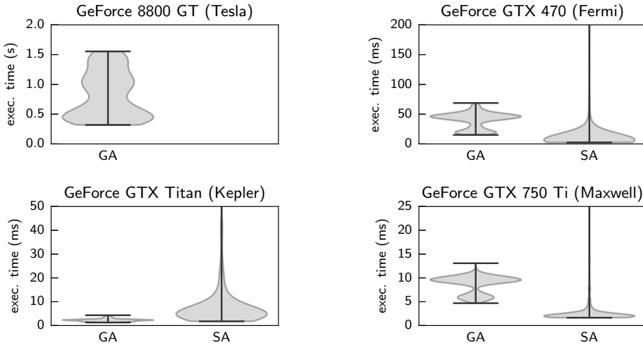
Figure 4.10: Distribution of execution times for the Hough transform in the polar coordinate system on four GPUs using either global memory atomics (GA) or scratchpad memory atomics (SA).
