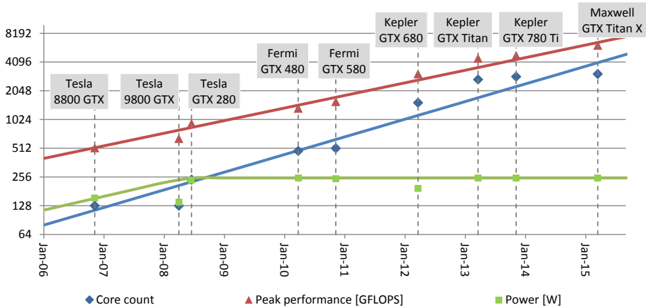
Figure 1.4: Core count, peak performance and maximum power consumption of various high-end GPUs at their time of introduction and their corresponding trend lines over the last 8 years.
