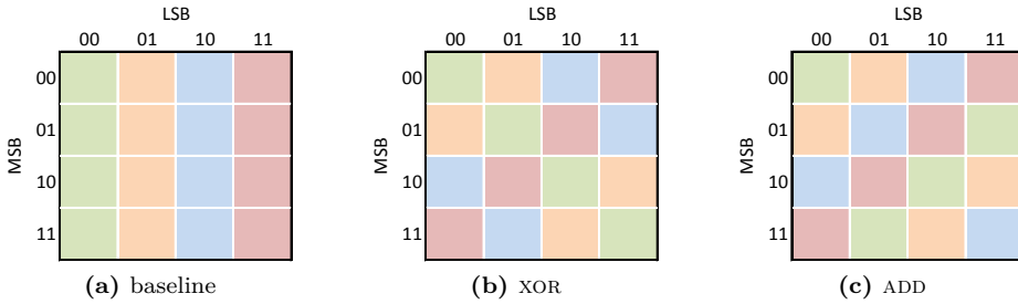
Figure 5.5: Overview of bank (and lock) distribution for three different hash functions, the different colors represent the four different memory banks. In (a) the baseline hash function is shown in which the LSB determines the bank. In (b) and (c) the XOR and ADD hash functions are shown in which the LSB are XORed / ADDED respectively with the MSB.
