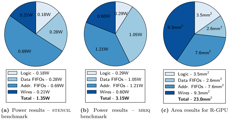
Figure 7.12: R-GPU power distribution in two benchmarks: memory bound (a) and compute bound (b) and the area distribution (c)
