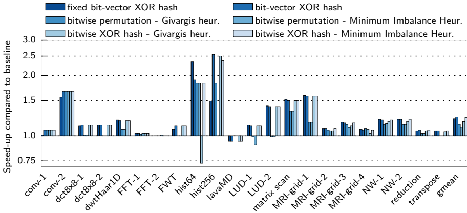
Figure 6.9: Overall speed-up obtained by the various hash functions compared to a baseline GPU (no hash function) for a set of benchmarks.
