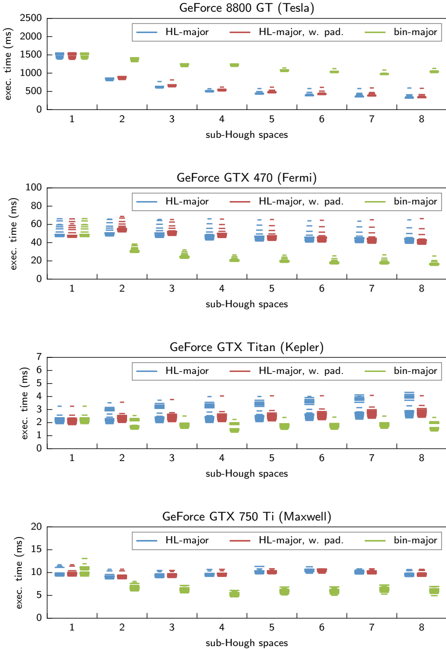
Figure 4.6: Hough transform on GPU using global memory atomic operations.
