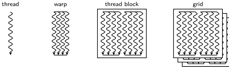
Figure 2.2: Hierarchy of threads, warps, thread blocks and grids in the CUDA programming model.
