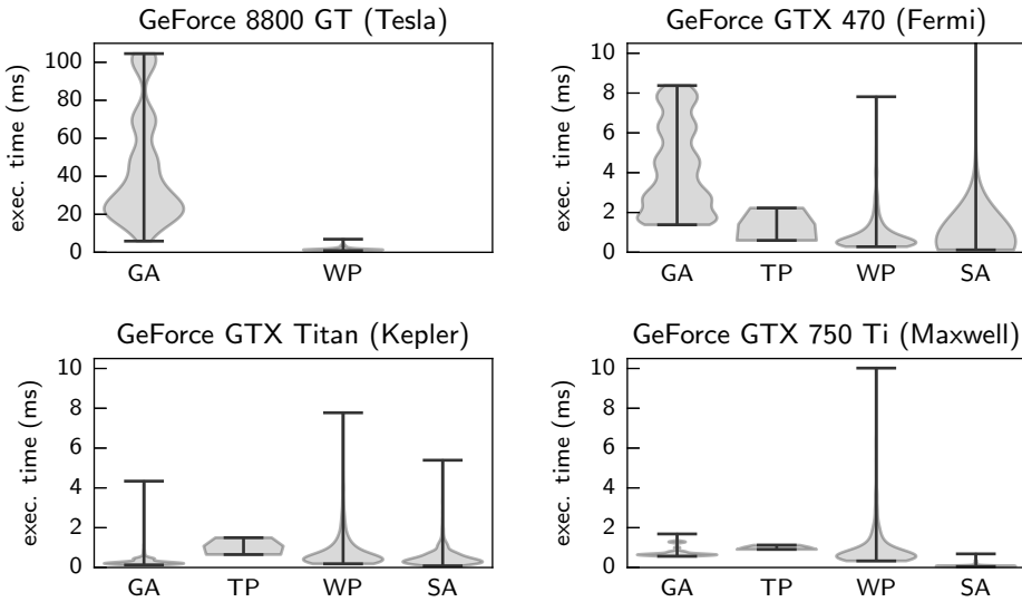
Figure 3.11: Distribution of execution times for a 256-bin histogram on four GPUs using either global memory atomics (GA), thread private sub-histograms (TP), warp private sub-histograms (WP) or scratchpad memory atomics (SA).
