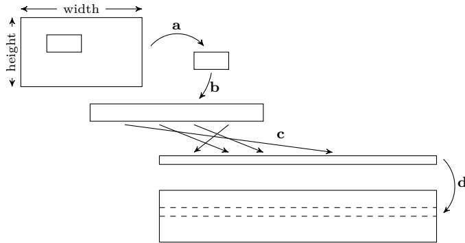
Figure 4.7: Fast implementation of the Hough transform on GPU. Each thread block in the first kernel converts a part of the image to an array of pixel coordinates in the scratchpad memory (a). The part of the array is added to the main array in global (off-chip) memory (b). In the second kernel the array of pixel coordinates is processed by a thread block to create one Hough line in the Hough space in the scratchpad memory (c). When the complete array of coordinates has been processed, the Hough line is copied to the Hough space in global memory (d).
