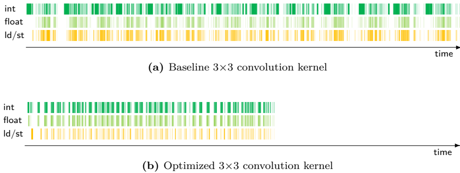
Figure 7.1: SM activity for (a) a baseline and (b) an optimized kernel. The activity is split into integer ( int ), floating point ( float ) and load-store ( ld/st ) operations.
