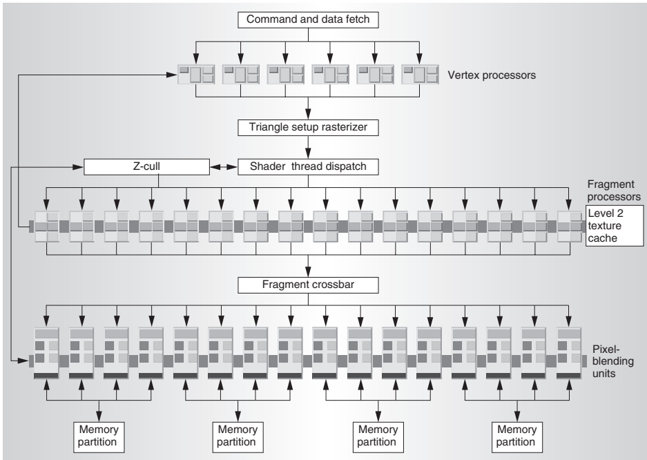
Figure 1.2: GeForce 6800 block diagram with 6 vertex processors, a rasterizer, 16 fragment processors and 16 pixel blending units. [61]
