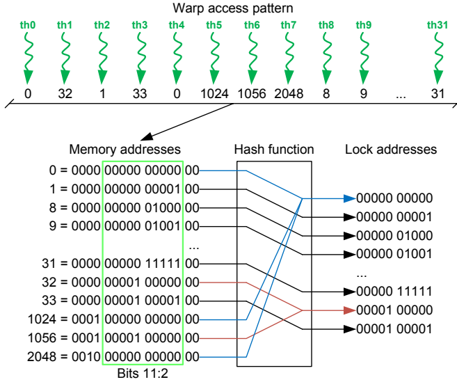
Figure 5.1: Hash function in lock mechanism. Given a memory address, the corresponding lock address is given by bits 11:2. Memory addresses at distance 1024 words are aliased, since they have the same lock address. This way, threads 0, 4, 5, and 7 will be executed sequentially, as well as threads 1 and 6.
