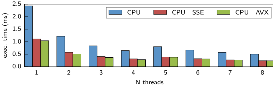
Figure 3.2: Execution time for calculating a 256-bin histogram on a CPU (Intel® Core™ i7-4770) using 1 to 8 threads
