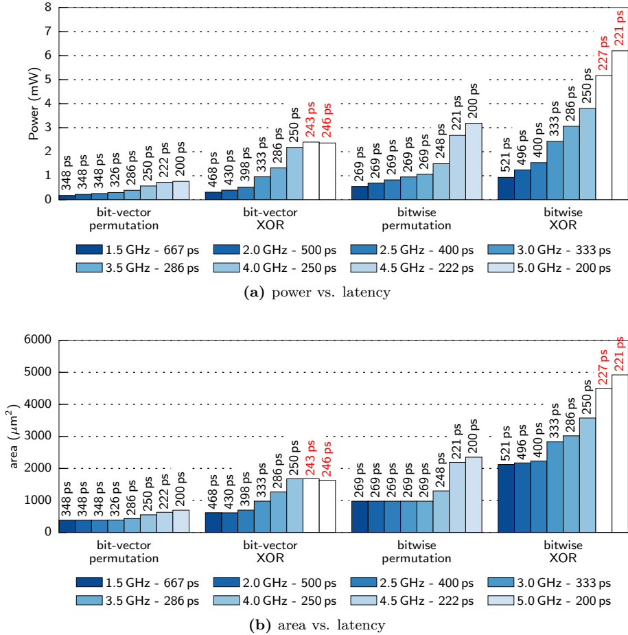
Figure 6.4: Power (a) and area (b) vs. latency results for the four proposed hash functions for a range of target clock frequencies (1.5 GHz – 5.0 GHz)
