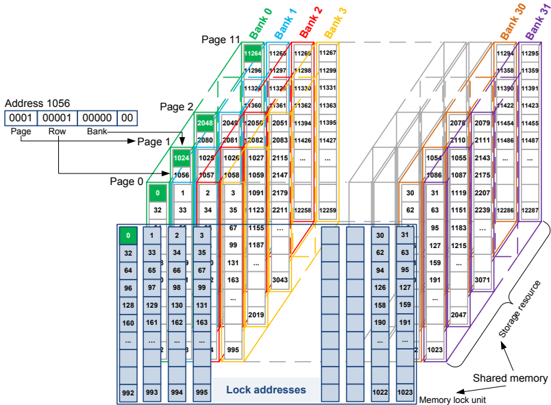
Figure 5.2: Scratchpad memory layout on an NVIDIA Fermi GPU. The 48 kB of memory is accessed via 4-byte words and is distributed over 32 banks. Each bank has 32 lock bits available for atomic operations.
