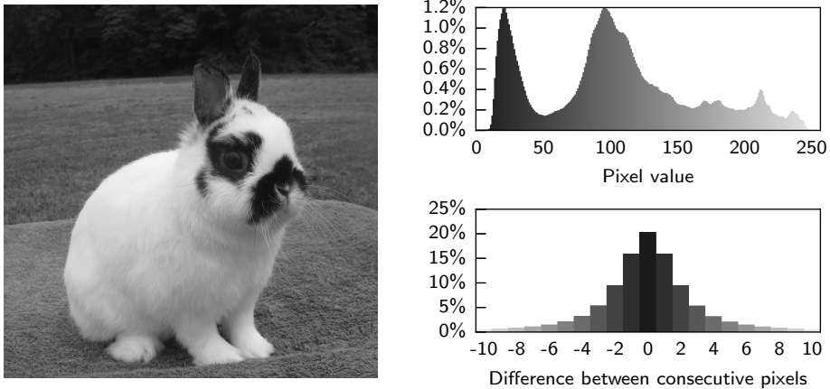
Figure 3.1: Image of a rabbit (left), the corresponding histogram (top right) and a histogram of the difference between consecutive horizontal pixels (bottom right).
