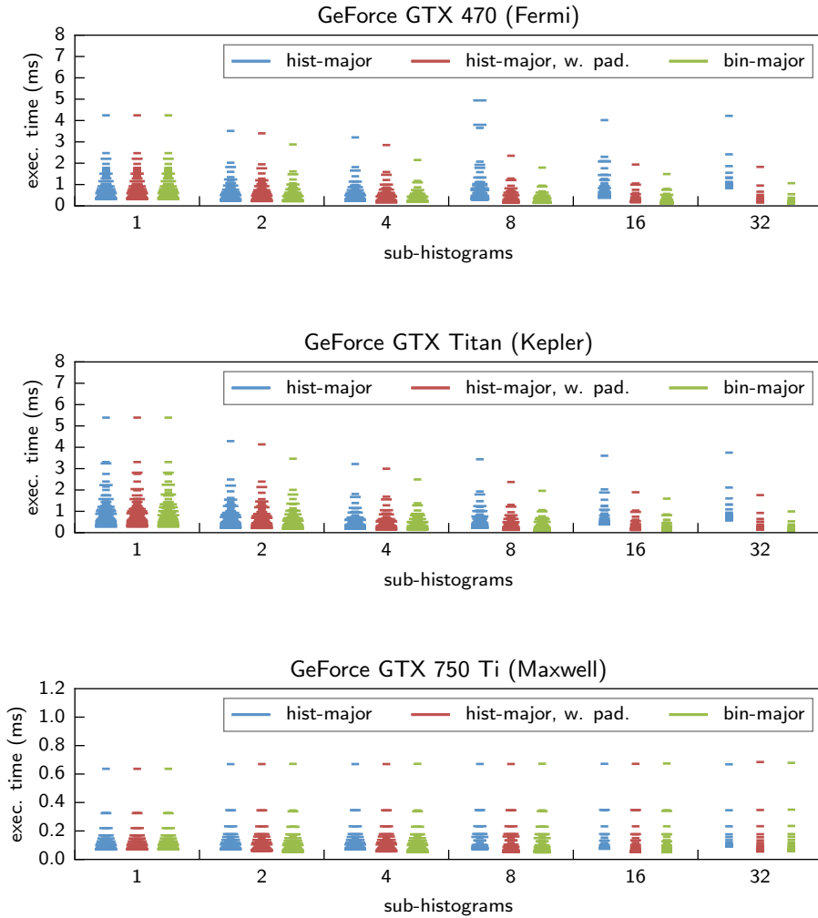
Figure 3.10: 256-bin histogram on four GPUs using atomic operations on scratchpad memory
