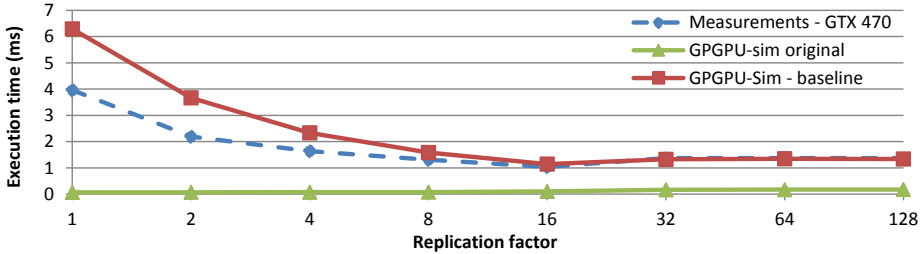
Figure 5.4: Comparison between measurements on an NVIDIA GTX 470, simulation results on the modified simulator and simulation results on the original GPGPU-Sim for a 64-bins histogram computation using a replication factor between 1 and 128 [25].
