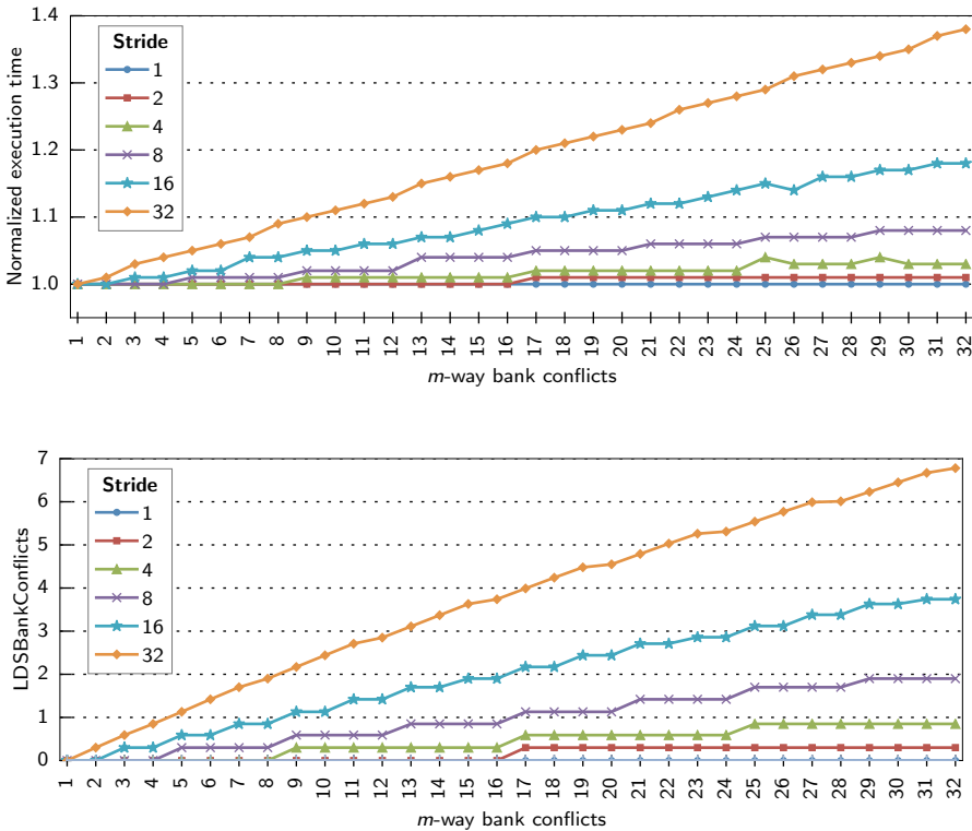
Figure 6.1: Execution results on AMD Hawaii for access patterns to scratchpad memory with different bank conflict degrees ( m -way) and strides. (Top) Normalized execution time; (Bottom) Profiling results.
