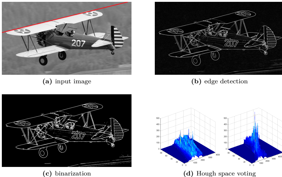
Figure 4.1: Test image of an airplane with the most dominant line (in red) found by the Hough transform (a); intermediate images after edge detection (b) and binarization (c); final Hough spaces (d).
