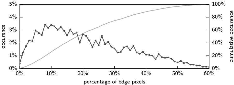
Figure 4.2: Distribution of the number of edge pixels in the images of the Van Hateren natural image database [110].
