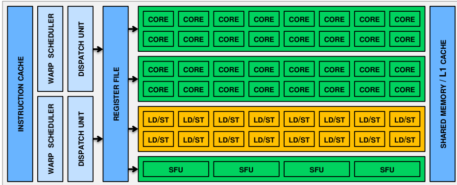
Figure 2.4: Streaming multiprocessor (SM) design of an NVIDIA Fermi GPU, consisting of two warp schedulers and two dispatch units, a register file, two groups of sixteen cores (CORE), one group of sixteen load-store units (LD/ST), one group of special function units (SFU) and a combined scratchpad (shared) memory and L1 cache.
