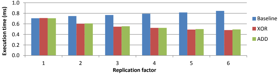
Figure 5.7: Hough transform (polar) on a 640 \times 480 image with six different replication factors (no padding) for the baseline, XOR and ADD hash function.
