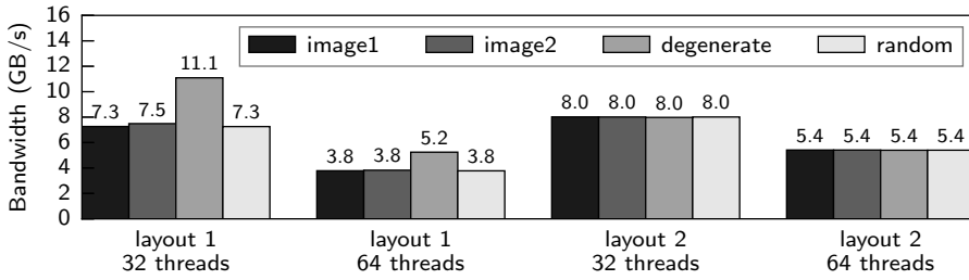
Figure 3.5: Results from [73] (Section 7) for a 256-bin histogram using a private sub-histogram per thread on a GeForce GTX 470. Two layouts are tested for four images, with either 32 or 64 threads per thread block.
