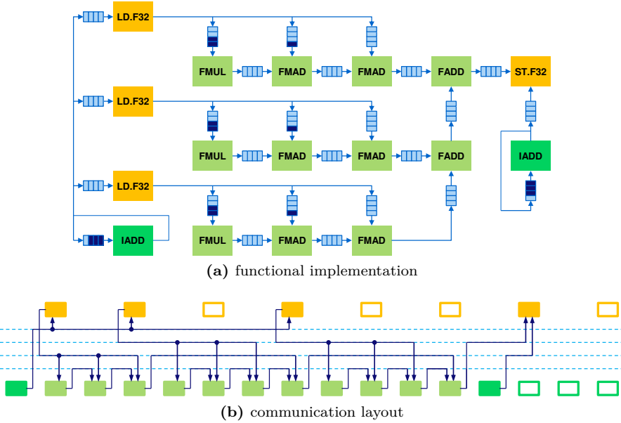
Figure 7.6: Functional implementation (a) and communication layout (b) for a 3 \times 3 2D convolution kernel in R-GPU. Cores with integer instruction are dark-green, those with floating point instruction in light-green. Cores and load-store units which are not active are shown as an outline only in the communication layout.
