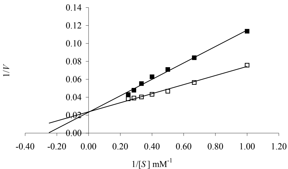
Fig. 4.3 Double reciprocal plots of the rate of hydrogen oxidation catalysed by membrane (A) and soluble fractions (B) of strain CBDB1 in the presence (■) and absence (□) of 75 \mu\text{M} \text{Ni}^{2+} . The reaction mixture contained 100 mM Tris-HCl buffer at pH 7.5 in the presence of a nominal concentration of 0.4 mM \text{H}_2 .
