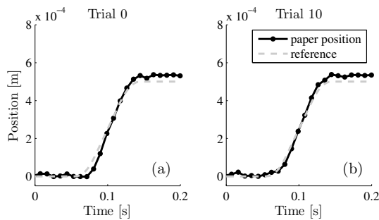
Fig. 9. Absolute paper position for the micro reference. In (a) the 0'th trial is shown, (b) shows trial 10. A small improvement in paper positioning is visible, note that the final paper position is too large for both trials.
