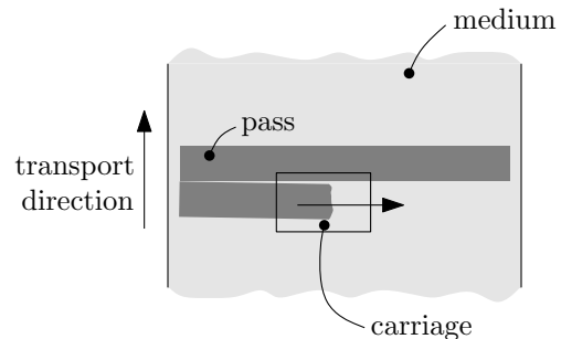
Fig. 1. Top view of the scanning inkjet printing process, showing unidirectional printing.
