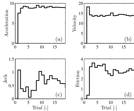
Fig. 11. The feedforward parameters for the macro trajectory as function of the trial number. It shows that the parameters converge to 90% of their final values in 2 trials.
