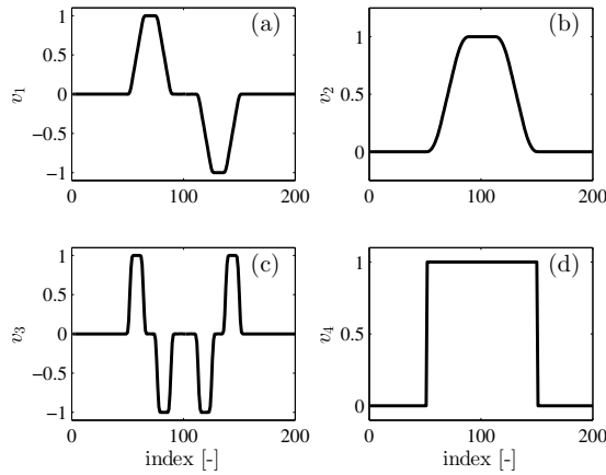
Fig. 6. The basis functions \Psi . Acceleration feedforward with basis function v_1 is shown in (a), velocity feedforward v_2 is shown in (b), plot (c) shows the Jerk feedforward and the basis function for Coulomb friction v_4 is shown in (d).
