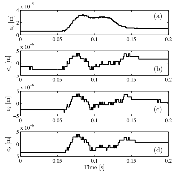
Fig. 7. Tracking errors for the micro reference for different trials. Trial 0 is shown in (a), (b) shows trial 1, and trial 2 and 5 are shown in (c) and (d) respectively. The tracking error converges after 1 trial of learning. The peak-peak error reduction is about a factor 8.
