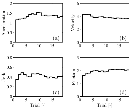
Fig. 8. The feedforward parameters for the micro trajectory as function of the trial number. It shows that the parameters converge to 90% of their final values in 1 trial.
