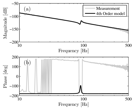
Fig. 5. Frequency response measurement of the plant with the derived 4th order model. The magnitude is shown in (a), the phase is shown in (b). There is good correspondence in the shown frequency range.
