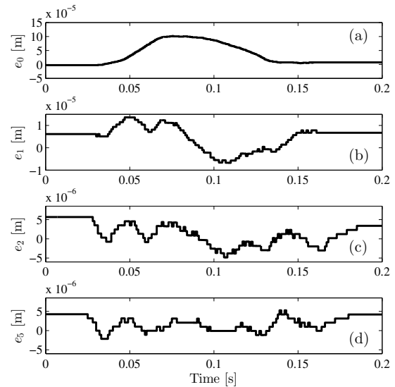
Fig. 10. Tracking errors for the macro reference for different trials. Trial 0 is shown in (a), (b) shows trial 1, and trial 2 and 5 are shown in (c) and (d) respectively. The tracking error converges after 2 trial of learning. The peak-peak error reduction is about a factor 20.
