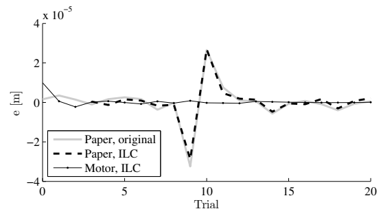
Fig. 12. Paper step error comparison. The original paper step error is shown in solid gray. The paper step error with ILC is shown in dashed black. The motor position error is shown in solid black with dots. There is a very small improvement in paper positioning error, note that the average of the error measurements on paper has been set to 0.
