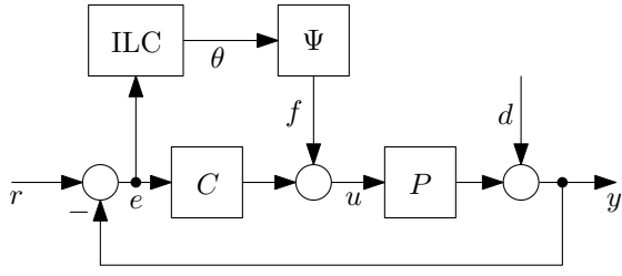
Fig. 4. Closed-loop system. The control loop consists of a standard linear feedback controller C which drives plant P with input u . The ILC updates the parameters \theta at the end of each trial. The feedforward f is constructed using the basis functions \Psi . The tracking error is e which is calculated using the positioning reference r and measured output y , which is affected by an unknown disturbance d .
