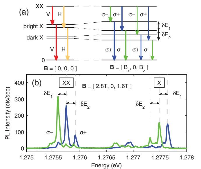
FIG. 3. (Color online) (a) Schematic of the neutral exciton and biexciton energy levels in a magnetic field at 60^\circ and (b) corresponding spectrum for B_{60} = 3.2 \text{ T} ( \mathbf{B} = [2.8 \text{ T}, 0, 1.6 \text{ T}] ).
