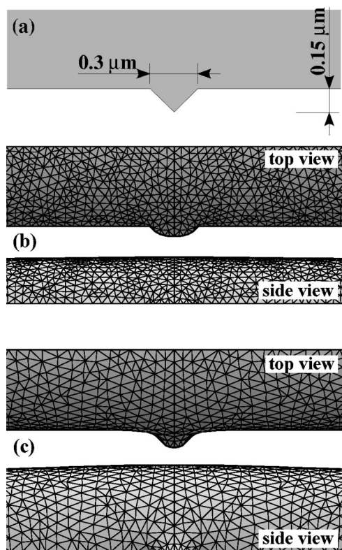
FIG. 9. Top- and side-view profiles of a liquid line on a hydrophilic channel of 1 \mu\text{m} width containing a triangular topological defect. The defect consists of a local protrusion of the channel boundary in the shape of an equilateral triangle with an apex angle of 90^\circ . The distance between the apex of the protrusion and the remaining channel boundary (the height of the triangle) is 0.15 \mu\text{m} . The deposited volumes are: (b) 0.2 \mu\text{m}^3 and (c) 0.4 \mu\text{m}^3 per unit length (in \mu\text{m} ). Only half of the liquid structure is shown in top view. In the vicinity of the inner corners of the triangle in (c), the liquid profile slightly overhangs and the top view does not show the actual liquid–solid contact line.
