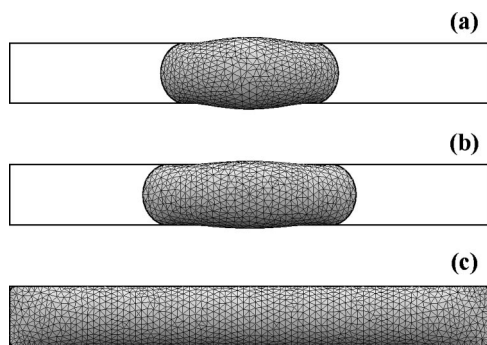
FIG. 7. Shape changes of a liquid droplet on a hydrophilic channel for different surface tensions but constant volume. The stripe has dimensions 1\ \mu\text{m} \times 8\ \mu\text{m} and is surrounded by completely hydrophobic regions. In (a) the droplet profile for a natural contact angle of 60^\circ is depicted. In (b) and (c) the influence of a surfactant is illustrated, which reduces the surface tension by (b) 20% and (c) 50% rendering the liquid completely wetting and enhancing the edge definition.
