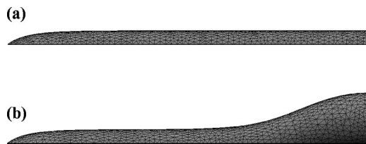
FIG. 3. Side-view profiles of liquid lines with a natural contact angle of \theta = 30^\circ on a hydrophilic stripe of dimensions 1 \mu\text{m} \times 16 \mu\text{m} surrounded by a completely hydrophobic surface. The liquid volume is increased from (a) 3.2 \mu\text{m}^3 to (b) 6.4 \mu\text{m}^3 .
