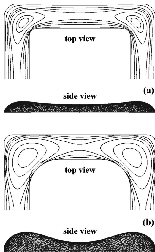
FIG. 5. Top- and side-view profiles for two different volumes of liquid on a hydrophilic channel forming a square loop of 1 \mu\text{m} width. The top view (a) depicts the equilibrium shape for 5 \mu\text{m}^3 , the bottom view (b) for 10 \mu\text{m}^3 . In both examples, the contact angle on the channel was chosen to be 45^\circ and the exterior angle 135^\circ . Only half of the entire loop is shown in top view. The contour levels are: (a) 0.01, 0.1, 0.2, 0.25, 0.29, 0.35, 0.4 and 0.42 \mu\text{m} , and (b) 0.01, 0.2, 0.3, 0.39, 0.5, 0.65, 0.75 \mu\text{m} .
