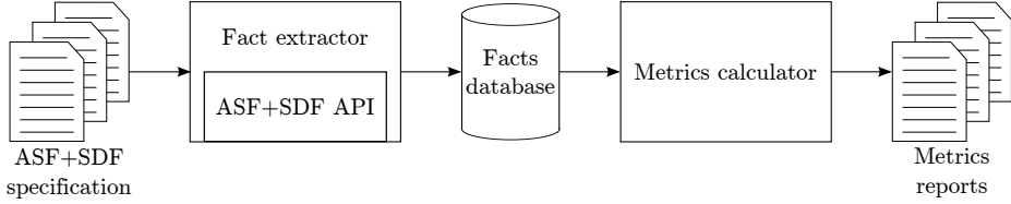
Figure 4.1 Tool architecture
