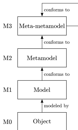
Figure 1.2 Four-layer metamodeling architecture
