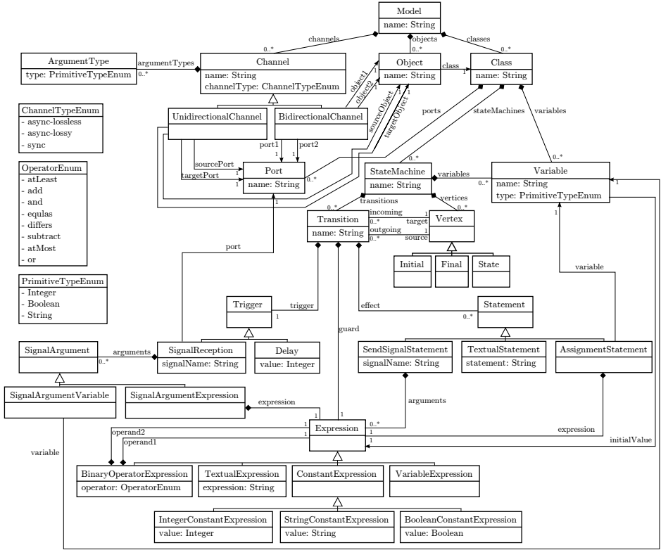
Figure 8.2 SLCO metamodel
