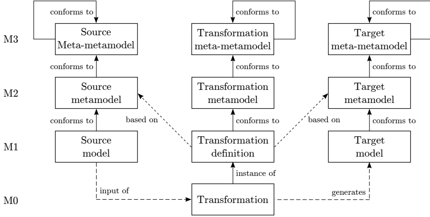
Figure 1.3 Transformation architecture
