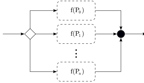
Figure 2.7 Alternative composition
