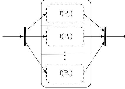
Figure 2.8 Parallel composition
