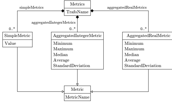
Figure 5.2 Metrics metamodel
