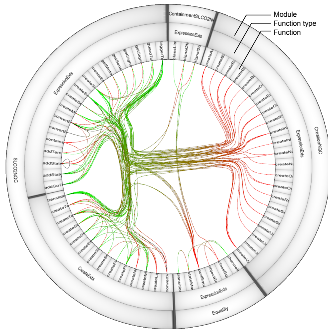
Figure 7.2 Trace visualization
