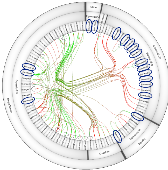
Figure 7.7 Using dependency analysis to detect obsolete transformation elements
