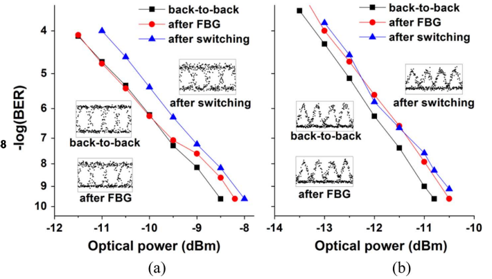
Fig. 9. BER curves of (a) 40 Gb/s NRZ packets and (b) 40 Gb/s RZ packets.
