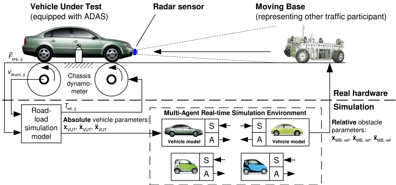
Fig. 1: VEHIL working principle.
