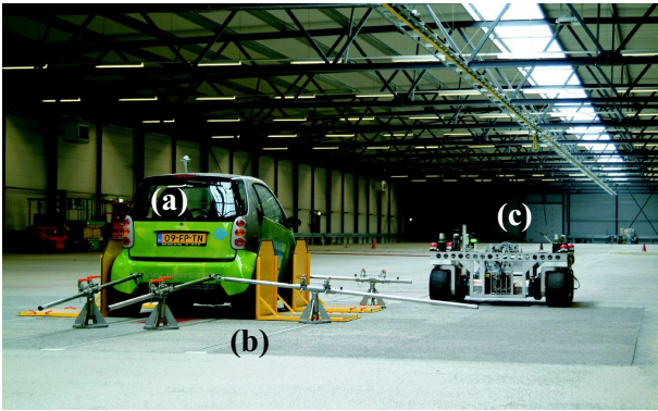
Fig. 3: VEHIL laboratory setup: (a) VUT equipped with a collision warning and avoidance system; (b) chassis dynamometer (beneath the floor) and (c) moving base.
