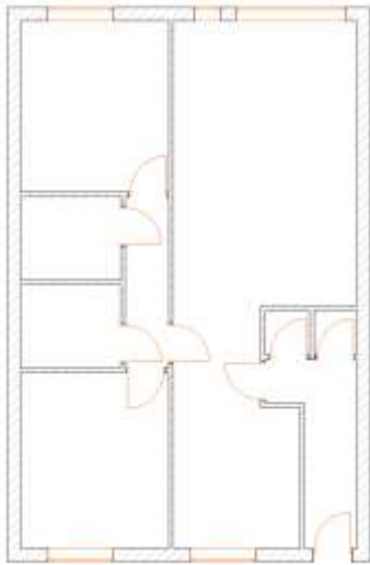
Figure 4. Apartment floor plan
