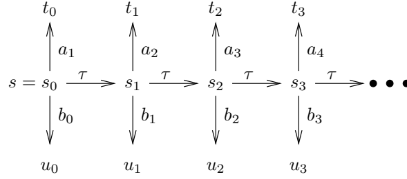
Figure 11. A divergence.
