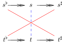
Figure 10. Stuttering closure.
