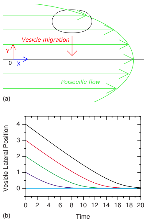
FIG. 1. (Color online) The plot (a) shows a schematic representation of the migration of a vesicle in a parabolic flow profile corresponding to an unbounded plane Poiseuille flow. The plot (b) shows the time evolution of the lateral position of a vesicle released initially at five different initial positions y_0=0,1,2,3,4 in units of the characteristic time \tau (right-hand plot).
