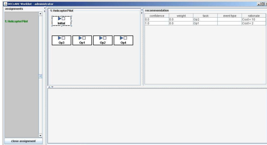
Fig. 7. Based on the data provided in the first step two operations are executable: Op1 and Op2 . Under a lowest cost strategy only Op1 is recommended (see upper right corner).
