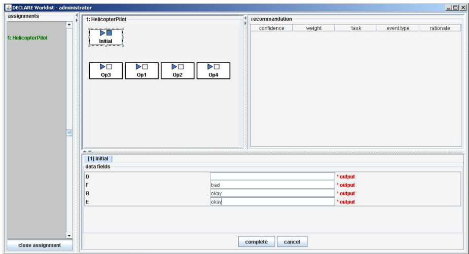
Fig. 5. As a first step a value for the input data elements has to be provided. In this example we have used the helicopter case again. A previous test result is not available ('D' is empty) and the other data elements are filled in.
