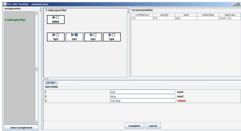
Fig. 8. The selected operation Op1 is executed by the user and the value for 'C' is added ('C'= 'not okay').
