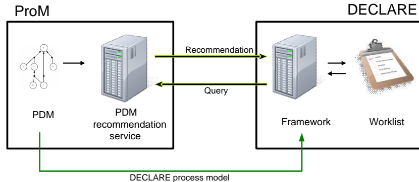
Fig. 4. An overview of the framework for PDM recommendations.
