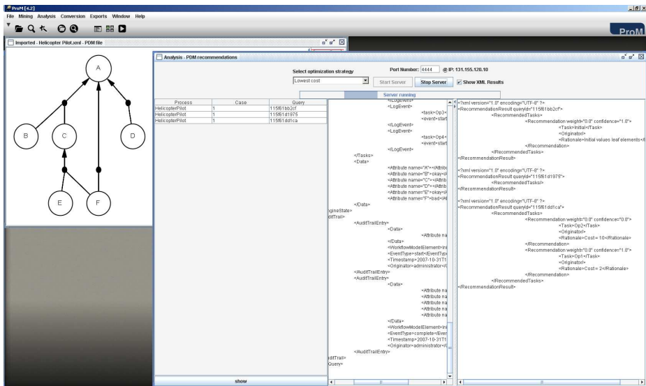
Fig. 6. The recommendation service calculates which operations are executable based on the availability of input elements. In this case only Op1 and Op2 are executable, since we have selected a lowest cost strategy Op1 is preferred over Op2 since the cost for the first one (2) are lower than for the second one (10).
