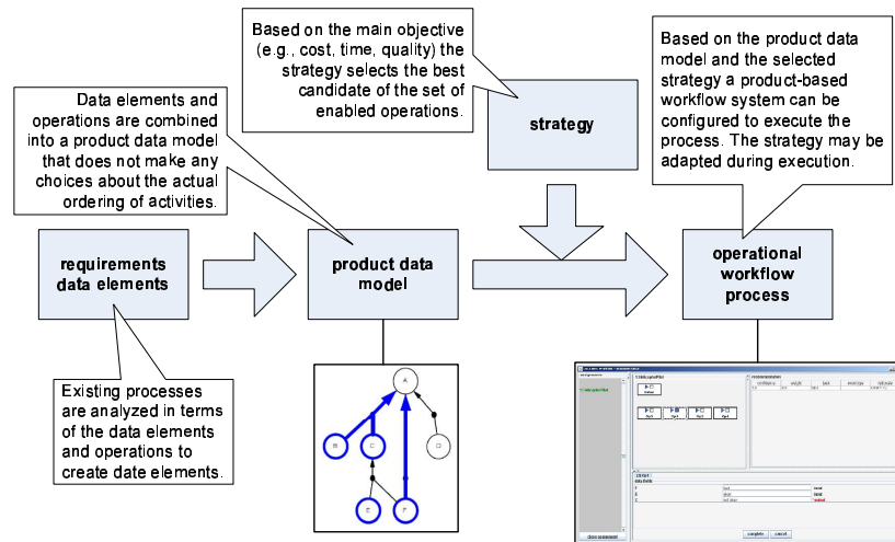
Fig. 1. Product Based Workflow Support (PBWS).
