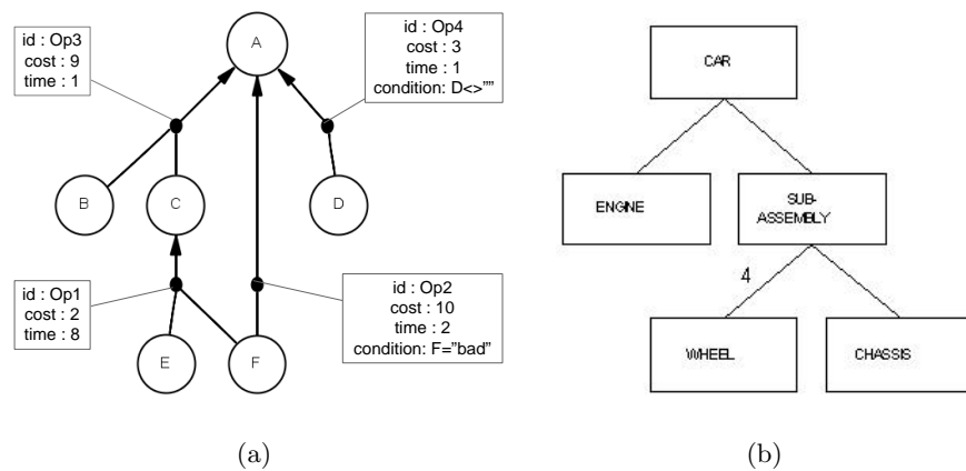
Fig. 2. (a) The product data model which represents the decision on the suitability to become a helicopter pilot. The meaning of the elements is as follows: (A) decision for suitability to become a helicopter pilot, (B) psychological fitness, (C) physical fitness, (D) latest result of suitability test in the previous two years, (E) quality of reflexes, (F) quality of eye-sight. Note that the operations have some attributes attached, such as an id and processing time. These attributes are important in selecting a suitable next step in the execution of the PDM for a specific case. (b) The Bill of Material (BOM) of a car with four wheels, a chassis and an engine.
