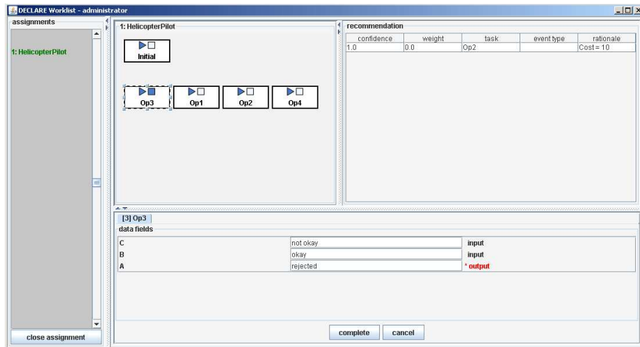
Fig. 10. The user executes Op3 and the end product A is produced. The process completes.
