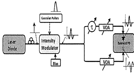
Fig. 3. Experimental setup
