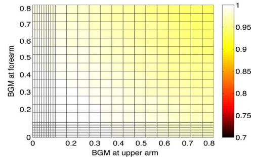
Fig. 11. Simulated recognition performance regarding BGM for a combination of acceleration and magnetic field sensors at forearm and upper arm.
