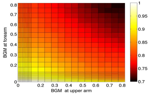
Fig. 10. Simulated recognition performance of rehabilitation postures (see Fig. 8) regarding BGM for acceleration sensors at forearm and upper arm.
