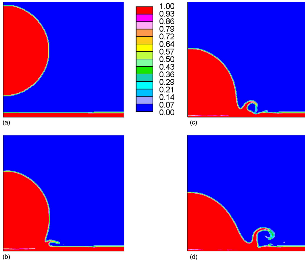
FIG. 15. (Color online) VOF fractions of an impacting water droplet with radius 100 \mu\text{m} and velocity 50 m/s on a 10 \mu\text{m} thick water film at times (a) t = 0.1 , (b) 1.5, (c) 2.0, and (d) 2.5 \mu\text{s} .
