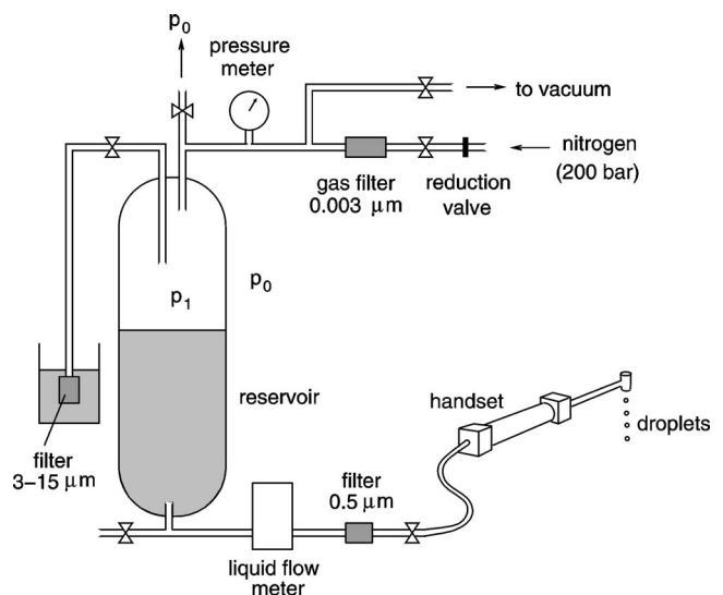
FIG. 1. Experimental setup to generate monodisperse droplets.
