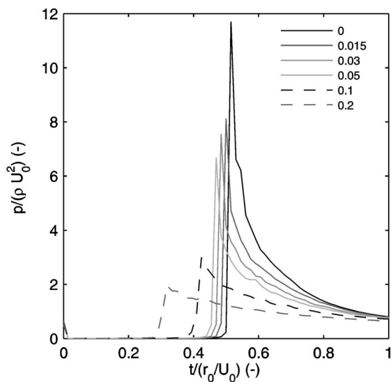
FIG. 16. The maximum dimensionless pressure along the solid surface during droplet impact as a function of the dimensionless time for different film thicknesses. The legend indicates the ratio between water layer thickness and droplet radius. A ratio of zero corresponds to impact on a dry surface. Droplet radius is 100 \mu\text{m} and droplet velocity is 50 m/s.
