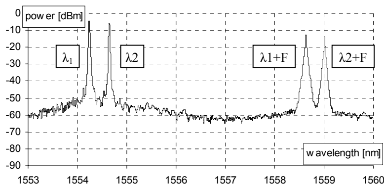
Figure 4. WDM signal transmitted from CO.
