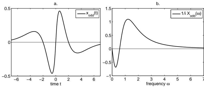
Figure 24: x_{\text{odd}}(t) and \frac{1}{i}X_{\text{odd}}(\omega) .
