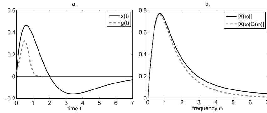
Figure 23: a. x(t) and a Gaussian window g . b. |X(\omega)| , and |X(\omega)G(\omega)| .
