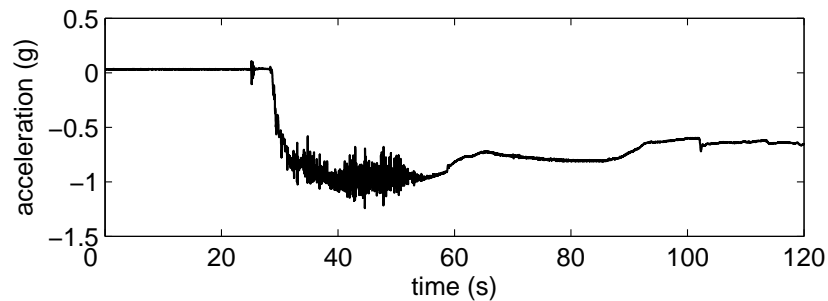
Figure 33: Example of motor seizure consisting of a mix of elementary patterns.
