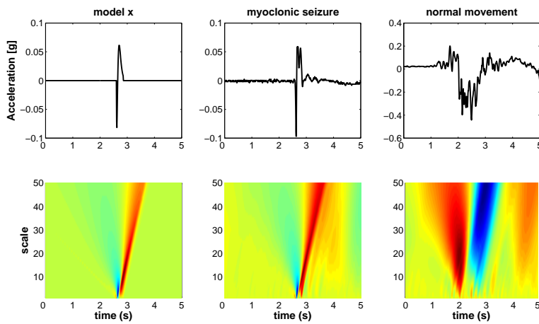
Figure 25: Wavelet transform of x , an accelerometric pattern that is associated with a myoclonic seizure, and an accelerometric pattern that is associated with a movement that is not a myoclonic seizure.
