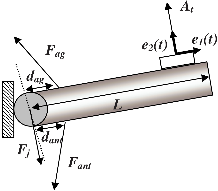
Figure 19: Schematic overview of the mechanical part of the model.
