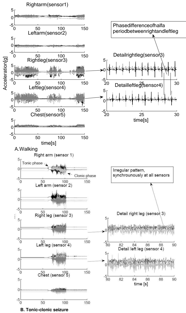
Figure 12: Pattern shape and context of all the sensors are important for distinguishing normal and epileptic patterns. A. Walking and B. Tonic-clonic seizure.
