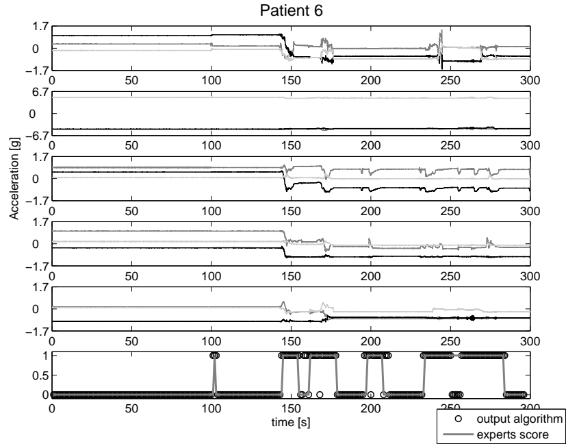
Figure 17: ACM-data of patient 6. The output of the algorithm and the experts score are plotted together in the last subplot. The value 0 indicates no motor activity whereas the value 1 indicates motor activity.
