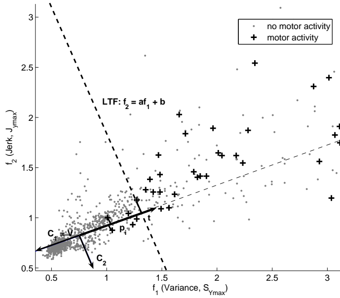
Figure 16: Graphical representation of computation of linear threshold function (LTF) in 2-D feature vector space. First the eigenvectors C_1 and C_2 of the covariance matrix of the cluster corresponding to 'no motor activity' are determined. The LTF is set perpendicular to the eigenvector corresponding to the largest eigenvalue V . The LTF is set in such a way that 98% of the 'motor activity' is on the right side of the LTF.
