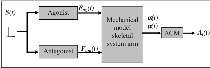
Figure 18: Schematic representation of model. S(t) is the innervation pattern sent from the central nervous system to the muscles. F_{ag}(t) and F_{ant}(t) represent the muscle force produced by the agonist and antagonist muscle. \omega(t) and \alpha(t) are the angular velocity and the angular acceleration of arm, and A_t(t) is the accelerometer output in the movement direction.
