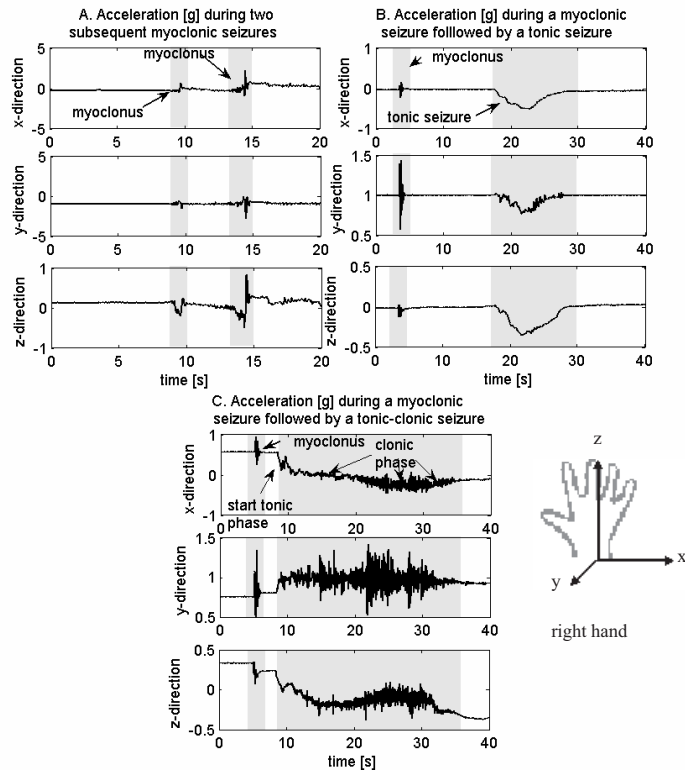
Figure 8: A. Typical pattern in the ACM-signal associated with a myoclonic seizure: a sudden shock-like movement of a short duration. B. Myoclonic seizure followed by typical tonic seizure pattern. The muscles are in tetanic contraction and the arm undergoes a slow change of posture. This results in a typical block-like pattern C. Myoclonic seizure followed by a typical tonic-clonic seizure pattern. During the clonic phase the arm is jerking repetitively, this results in a typical burst-like pattern. These signals are obtained from one 3-D sensor, placed at the right wrist. x-, y-, and z-directions are defined as depicted in the picture of the hand.
