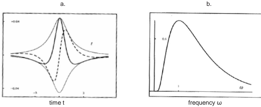
Figure 22: Bessel wavelet x(t) = \frac{1}{\pi\sqrt{1-it}} K_1(2\sqrt{1-it}) (imaginary part dashed), with K_1 a modified Bessel function of order 1, and its Fourier transform X(\omega) = e^{-(\omega+1/\omega)} , \omega > 0 , from [113].
