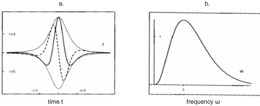
Figure 21: Cauchy wavelet x(t) = \frac{1}{2\pi(1-it)^3} (imaginary part dashed), and its Fourier transform X(\omega) = \omega^2 e^{-\omega} , from [113].
