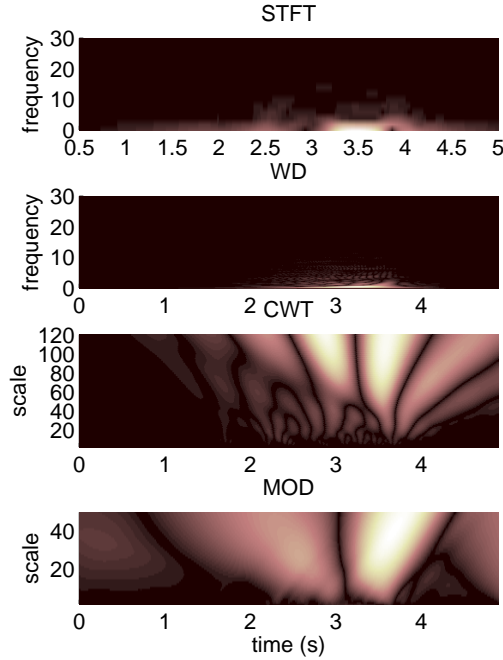
Figure 29: Time-frequency representations of normal movement. For STFT and WD, most of the power is concentrated in the lowest frequency band. For CWT and MOD we see high powers in the higher scales (low frequencies).
