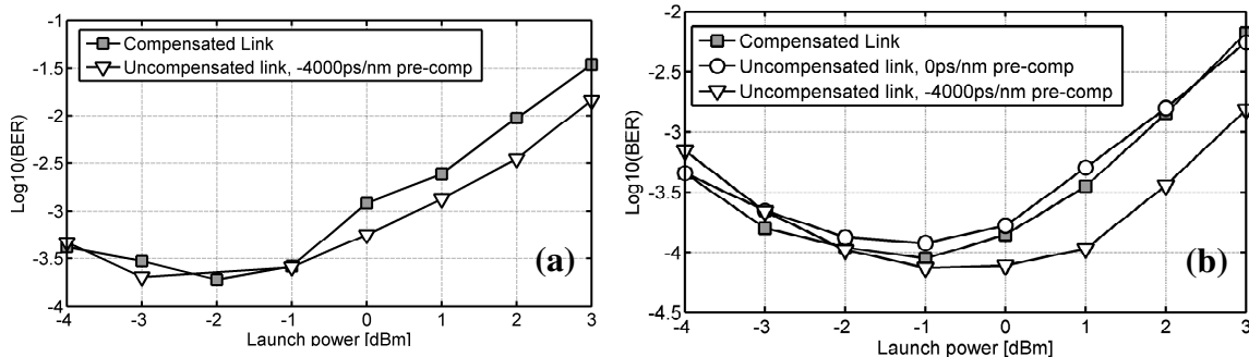
Fig. 5: Transmission performance w/ and w/o optical dispersion compensation, neighbors at: (a) 50-GHz and (b) 200-GHz spacing.
