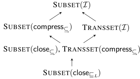
Figure 4: The lattice of algorithms presented in the previous sections.
