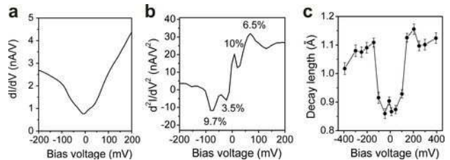
FIG. 3. Averaged dI/dV (a) and d^2I/dV^2 (b) spectra taken on graphene monolayer on SiC(0001) and its tunnel current decay length \lambda as a function of bias voltage (c). An inelastic peak intensity \Delta\sigma/\sigma is indicated at the each attributed phonon peak in d^2I/dV^2 . Scanning parameters: 64 \times 64 grid, V = 50 mV and I = 70 pA. The decay lengths have been determined from I(z) spectroscopy at fixed bias voltage by fitting it by an exponential function I(z) = \exp(-z/\lambda) . Error bars represent standard deviations of the measurements.
