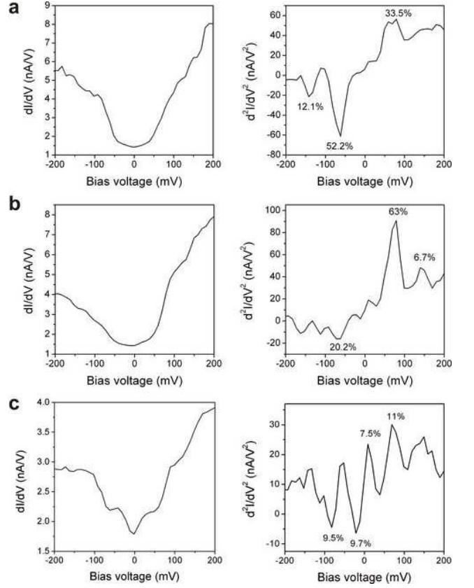
FIG. 5. dI/dV and d^2I/dV^2 spectra on graphene monolayer on SiC taken at V = 50 \text{ mV} and I = 50 \text{ pA} . The spectra represent typical individual dI/dV and d^2I/dV^2 curves obtained in red regions (a), blue regions (b) and gray regions (c) in Figure 4. Inelastic peak intensities \Delta\sigma/\sigma are indicated at the each attributed phonon peak in d^2I/dV^2 .
