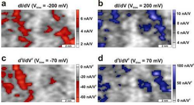
FIG. 4. (Color online) dI/dV (a,b) and d^2I/dV^2 (c,d) maps at constant bias voltage indicated in the right top corner of a 12 \times 8 \text{ nm}^2 area on graphene monolayer on SiC(0001). Red regions indicate high intensity inelastic phonon contributions at -70 \text{ mV} and high dI/dV at -200 \text{ mV} and blue regions mark out high intensity d^2I/dV^2 at 70 \text{ mV} and dI/dV at 200 \text{ mV} . Scanning parameters: V = 50 \text{ mV} and I = 50 \text{ pA} .
