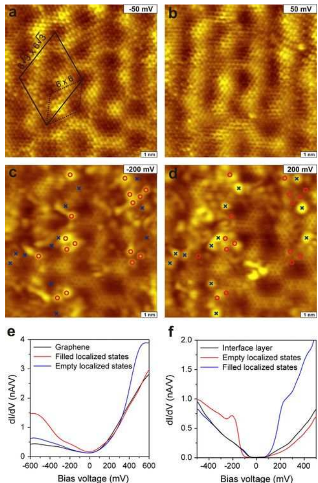
FIG. 2. (Color online) STM images of a 10 \times 10 nm 2 area on single-layer graphene on SiC(0001) taken with I = 5 pA and V = -50 mV (a), 50 mV (b), -200 mV (c) and 200 mV (d). Circles point out the positions of the bright dots in the filled states and crosses in the empty states. (e) Three local characteristic dI/dV spectra on monolayer graphene on SiC(0001) ( V = 300 mV and I = 41 pA). (f) Three local characteristic dI/dV spectra on the interface layer on SiC(0001) ( V = -200 mV and I = 5 pA). All STS curves have been averaged over 10 curves.
