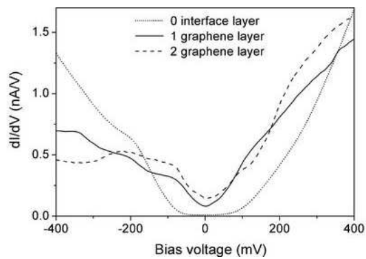
FIG. 1. Spatially averaged STS curves on the 0 interface, 1st and 2nd graphene layers on SiC(0001). Scanning parameters: V = -200 mV, I = 50 pA for graphene monolayer and bilayer, and V = -200 mV, I = 5 pA for the 0 layer.
