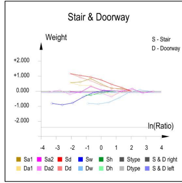
Figure 11. Curves of Stair-Doorway
