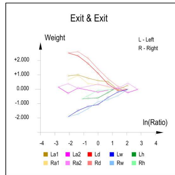
Figure 10. Curves of Exit-Exit
