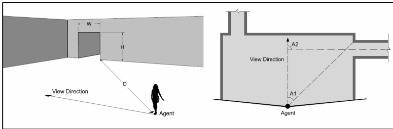
Figure 2. Variables of Doorway
