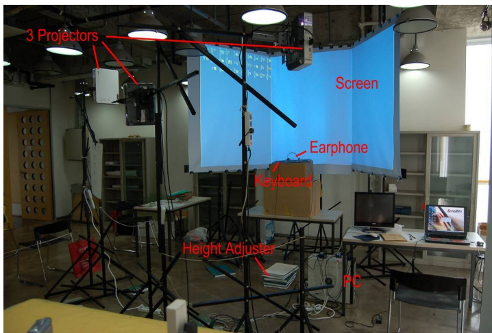
Figure 5. The CAVE for the experiment
