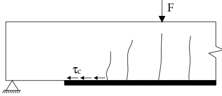
Figure 9: Debonding at the end anchorage
