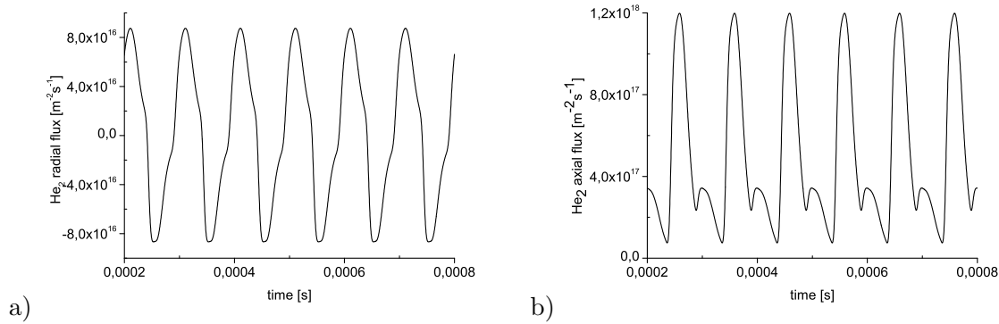
Figure 6. Calculated a) radial and b) axial fluxes of He 2 for a mass flow rate of 5 l/min. The applied voltage frequency and amplitude are 10 kHz and 2.6 kV. The gap width is 0.7 mm.
