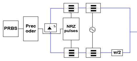
Figure 2 DQPSK RZ transmitter
