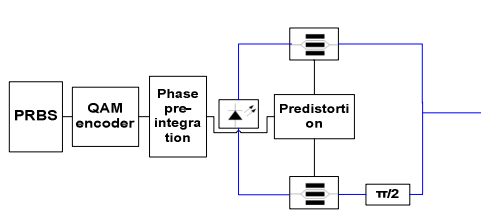
Figure 1 QAM transmitter
