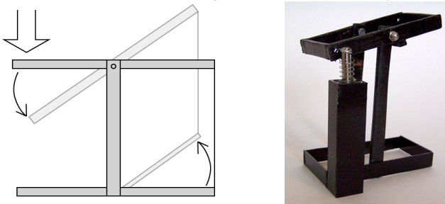
Figure 3. Iconic bridge, schematic (left) and prototype (right).
