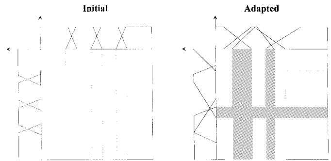
Fig. 1. Fuzzy partition of two premise variables. Adapting the fuzzy sets which define an initial fuzzy partition for the premise space can result in similar fuzzy sets.
