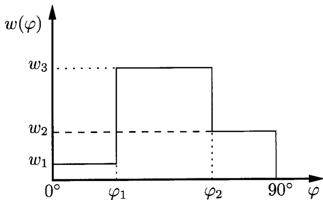
FIG. 7. Weight function to emphasize the region over which the optimization is carried out.
