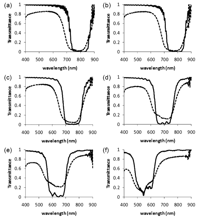
FIG. 3. Transmission spectra for unpolarized light of a configuration with a half-lambda plate sandwiched between two right-handed CLC layers. The pitch varies linearly from 464 to 523 nm in the layers. The refractive indices are n_e=1.68 and n_o=1.54 . The half-waveplate has a center wavelength of 825 nm. Dashed lines indicate the experimental measurements, solid lines indicate calculations. Figures (a) to (f) are for incident angles in glass of 0^\circ , 10^\circ , 20^\circ , 30^\circ , 40^\circ , and 50^\circ , respectively.
