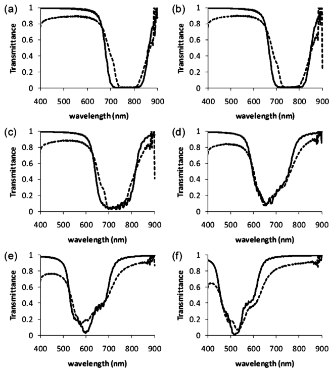
FIG. 2. Transmission spectra for unpolarized light of a right-handed CLC stacked on top of a left-handed CLC. The pitch varies linearly from 437 to 520 nm in the right-handed material and from 429 to 521 nm in the left-handed material. The refractive indices, n_e=1.68 and n_o=1.54 , are the same for both materials. Dashed lines indicate the experimental measurements, solid lines indicate calculations. Figures (a) to (f) are for incident angles in glass of 0^\circ , 10^\circ , 20^\circ , 30^\circ , 40^\circ , and 50^\circ , respectively.
