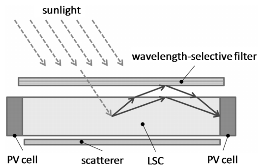
FIG. 1. (Color online) LSC lightguide with wavelength-selective filter (which may be attached to the LSC) and scatterer. PV cells are attached to one or more of the lightguide edges. Sunlight passes through the filter, but the luminescent light is reflected.
