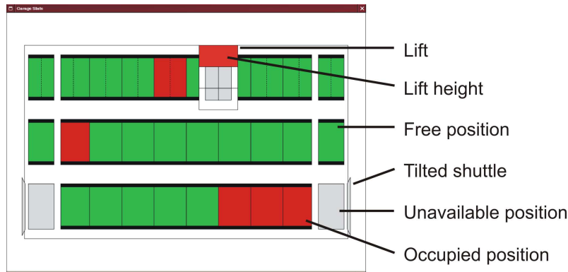
Figure 6: Visualization plug-in
