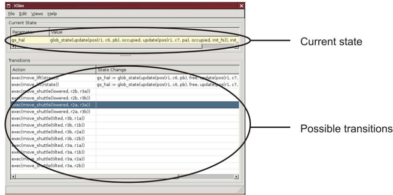
Figure 4: Simulator
