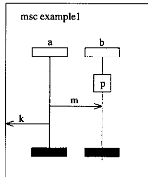
Figure 2: Example Basic Message Sequence Chart
