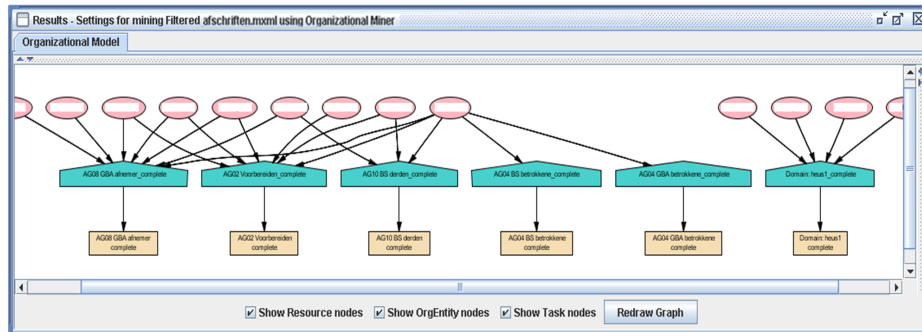
(c) Organizational model: the 6 roles and 13 originators are discovered
