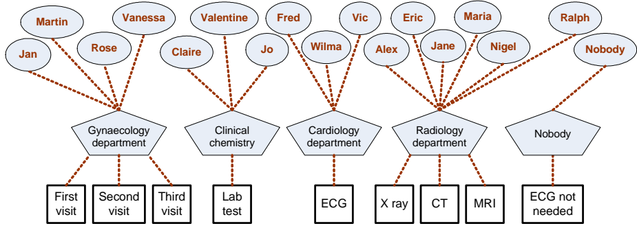
Fig. 8. Example model enhanced with the organizational perspective. The boxes represent activities, the pentagons represent roles, and the circles represent originators
