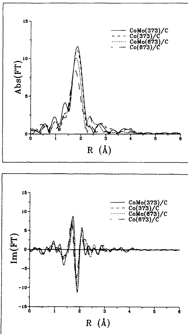
Figure 2. Absolute value and imaginary part of the FT spectra of the k^3 -weighted EXAFS functions of the four samples. The spectra have not been phase- and amplitude-corrected.
