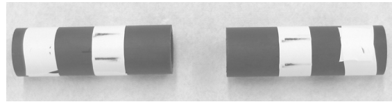
Fig. 23. Fractured specimen 2
