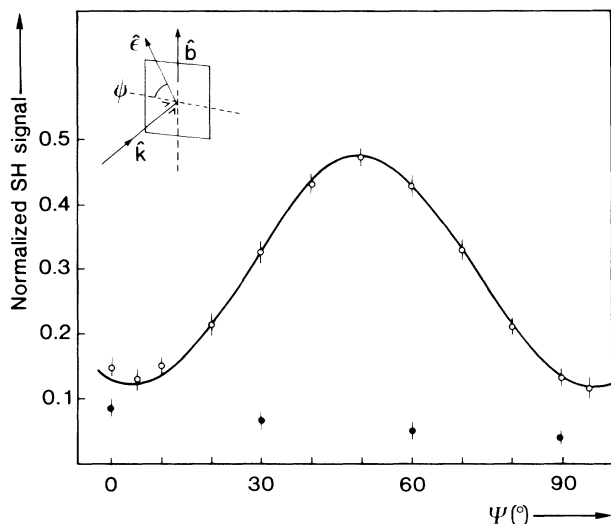
FIG. 1. The intensity of SHG vs \psi , the angle between the crystal c axis and the linear polarization of the fundamental wave, incident perpendicularly to the b - c plane. The SHG measured with the analyzer parallel to the crystal b axis is given with the open symbols, while the closed symbols represent the SHG measurements with the analyzer parallel to the c axis. The solid line represents the calculated function \sin^2(2\psi) , with a small offset in \psi that is within the experimental uncertainty.
