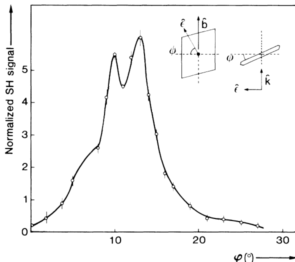
FIG. 2. The intensity of SHG vs the angle \phi of the rotation around the b axis of the crystal, with \psi = 45^\circ .
