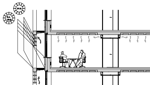
Figure 1: Principle of the shading and of the nighttime forced ventilation.
