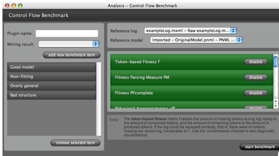
Fig. 4. Screenshot of the Control Flow Benchmark settings. A set of models can be selected to be compared with respect to a log and/or a reference model based on a number of different metrics
