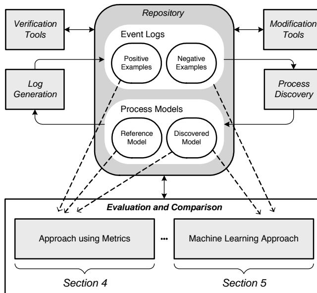
Fig. 3. Outline of a possible evaluation framework
