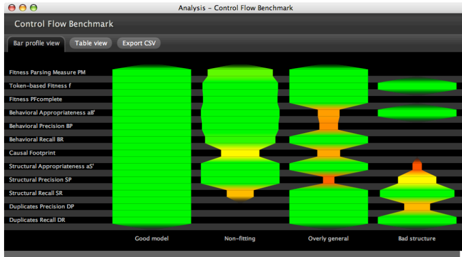
Fig. 5. Screenshot of the Bar Profile view in the Control Flow Benchmark plug-in in ProM. The visualization of the metric values provides an overview, and makes it easy to spot problems
