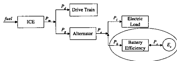
Fig. 1. Block diagram of vehicle's power flow
