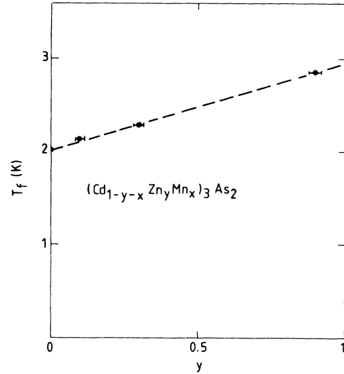
FIG. 12. Freezing temperature T_f as a function of the Zn concentration at constant ( x=10 at. %) Mn concentration in (\text{Cd}_{1-y-x}\text{Zn}_y\text{Mn}_x)_3\text{As}_2 .
