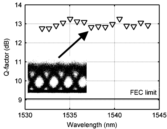
Fig. 7. Q -factors of all 16 WDM channels.
