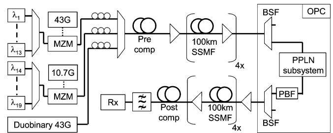
Fig. 8. Experimental setup of WDM 42.7-Gb/s NRZ, 42.7-Gb/s duobinary and 10-Gb/s NRZ transmission.
