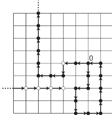
Figure 1: The arrows and the colors represent an element \eta of \Omega_\Lambda , where \Lambda = \{-3, -2, -1, 0\} , the set of possible steps is F = \{\rightarrow, \uparrow, \leftarrow, \downarrow\} and the set of possible scenery values is G = \{\circ, \bullet\} . The picture corresponds to \eta_n = (\rightarrow, \circ) for n \in (-\infty, -4] \cap \mathbb{Z} , \eta_1 = (\downarrow, \bullet) , \eta_2 = (\downarrow, \bullet) , \eta_3 = (\leftarrow, \bullet), \dots , \eta_{14} = (\leftarrow, \circ) , \eta_{15} = (\downarrow, \bullet) , \eta_{16} = (\leftarrow, \bullet) , \eta_{17} = (\leftarrow, \bullet) , \eta_n = (\uparrow, \bullet) for n \in [18, \infty) \cap \mathbb{Z} .
