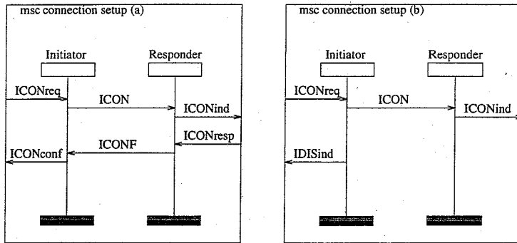
Figure 1. Two Message Sequence Charts
