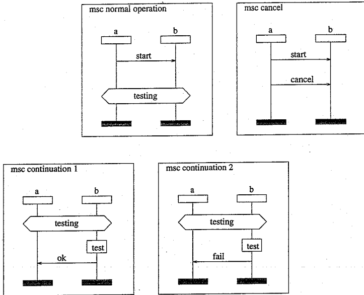
Figure 3. Example Message Sequence Charts
