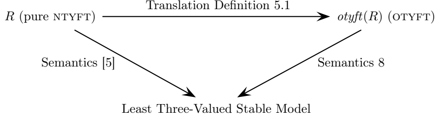
Figure 2: Soundness of the Translation from the pure NTYFT format to the OTYFT format
