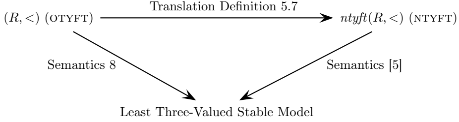
Figure 3: Soundness of the Translation from the OTYFT format to the NTYFT format
