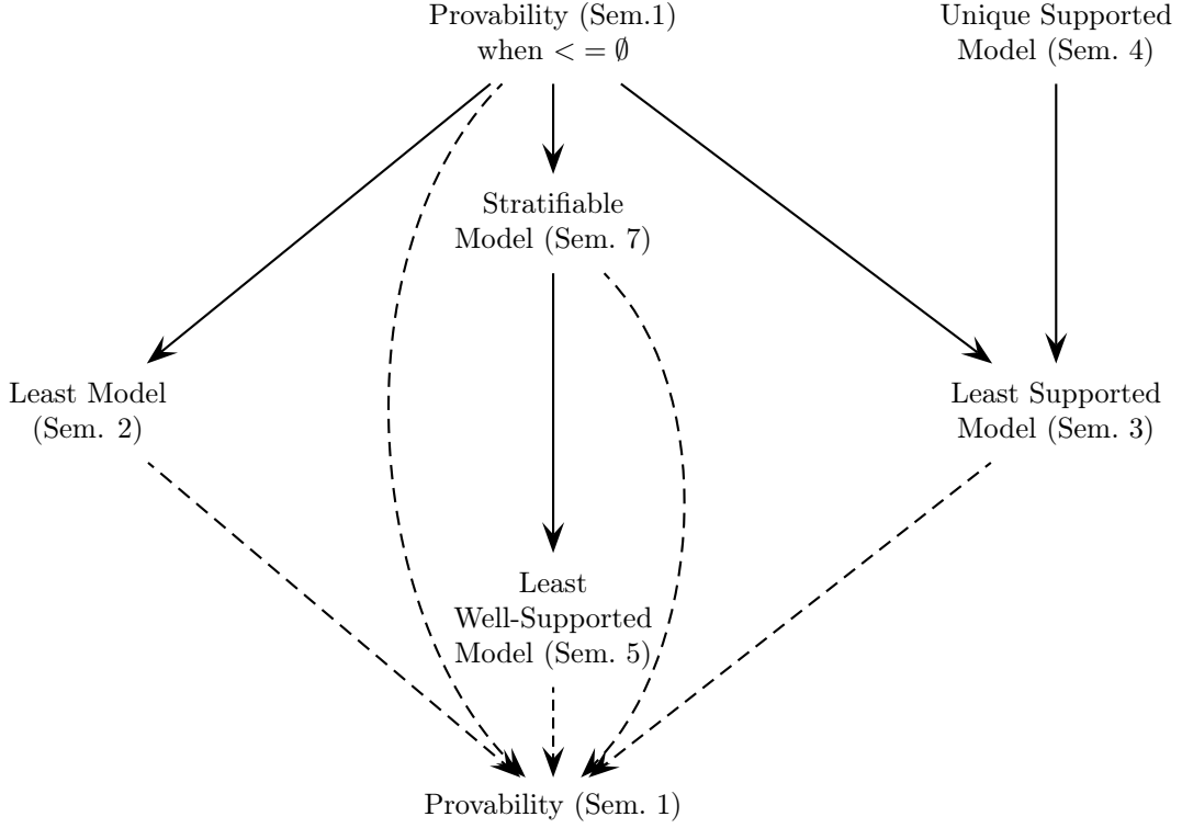
Figure 1: A Comparison of the Two-Valued Notions of Semantics
