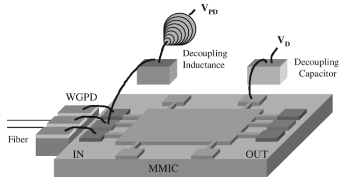
Fig. 10. Schematic representation of a hybrid photoreceiver.
