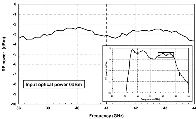
Fig. 11. Frequency response of the 40-GHz hybrid module.
