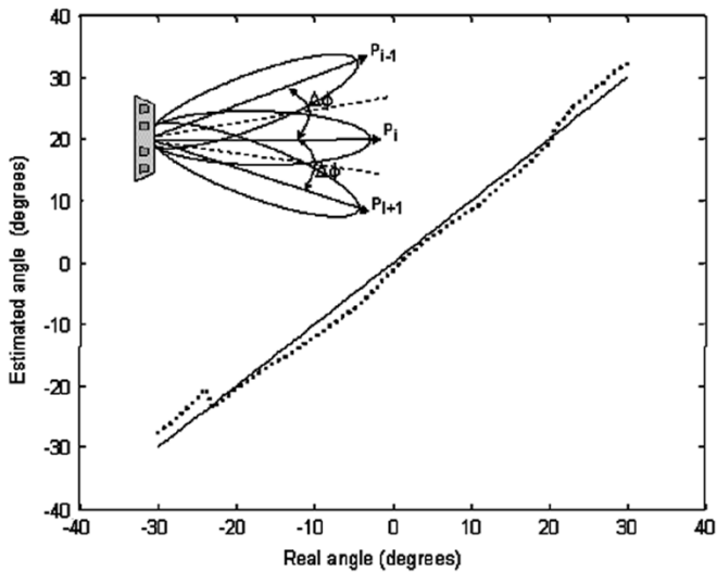
Fig. 23. Estimated angle as a function of the real angle of the terminal. The dotted line corresponds to the experimental results while the solid line depicts the ideal performance. The inset shows the schematic of the proposed DOA algorithm.
