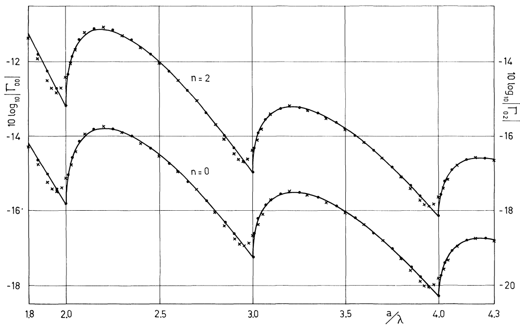
FIG. 3. Reflection coefficient amplitude for TM_{0n} mode, with TM_{00} mode incident (continuation of Fig. 2). Legend: as in Fig. 2
