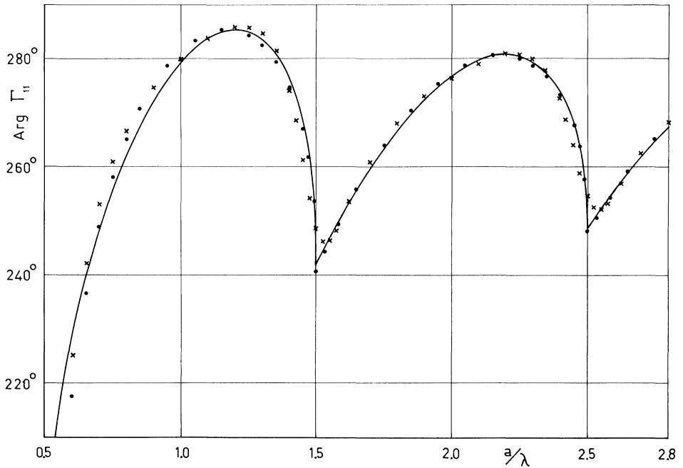
FIG. 7. Reflection coefficient phase for TM_{01} mode, with TM_{01} mode incident. Legend: as in Fig. 2
