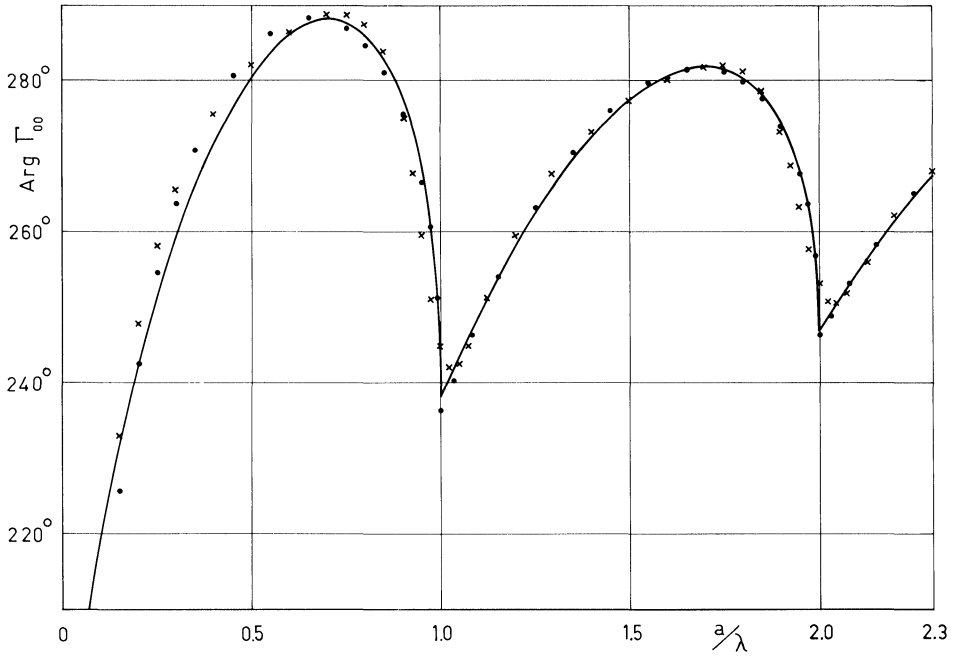
FIG. 4. Reflection coefficient phase for \text{TM}_{00} mode, with \text{TM}_{00} mode incident. Legend: as in Fig. 2
