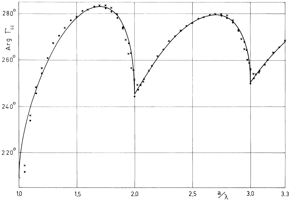
FIG. 5. Reflection coefficient phase for \text{TM}_{02} mode, with \text{TM}_{00} mode incident. Legend: as in Fig. 2
