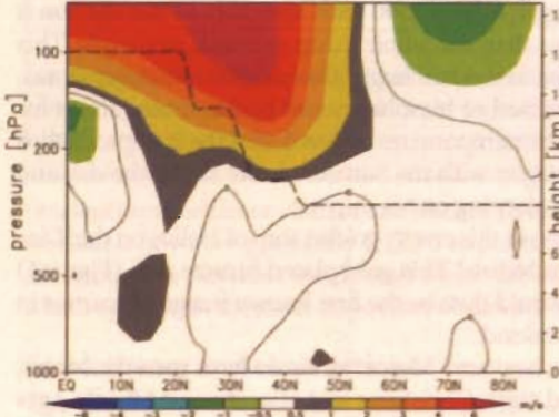
b) westerly wind response (stratospheric CO 2 doubling)
