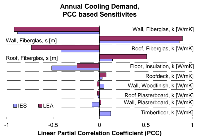
Figure 4: Annual Energy Demand for Cooling, PCC based Sensitivities, Comparison IES – LEA.
