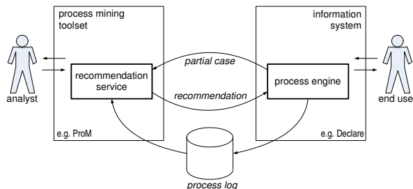
Fig. 2. An overview of the recommendation service.
