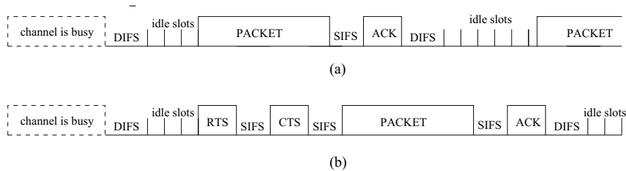
Figure 1: The IEEE 802.11 access mechanisms: (a) Basic access mechanism; (b) RTS/CTS mechanism.
