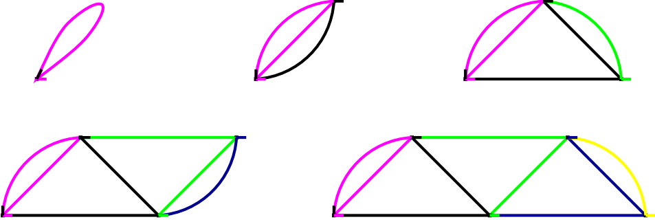
Figure 1 The diagrams for \pi_m^{(N)} , N = 1, \dots, 5 , arising from the expansion and the bound (3.28) for both models. The subwalks (indicated by different shades) in the diagrams have the previous subwalk as their history. An intersection of two subwalks and a small factor \beta appears at each vertex.
