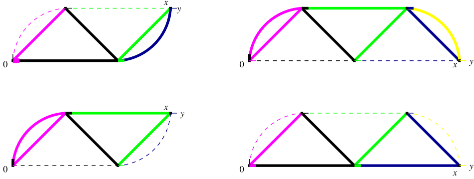
Figure 2 Illustration of the four cases of the diagrammatic bounds for OERRWD. On the left N is even ( N = 4 ) and on the right N is odd ( N = 5 ). In the first row \vec{j} \in B_0 , while in the second, \vec{j} \in B_1 \setminus B_0 . In each case the thick lines indicate the loops (whose total length is of order half of the total length m of the diagram) that give an exponentially small bound.
