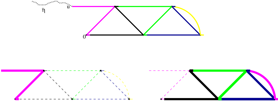
Figure 3 A diagrammatic representation of \Pi_m^{(N), \vec{\eta}}(u) for N = 5 , followed by the decomposition of the diagram when j_1 > m/2 and when j_1 \leq m/2 respectively. In each case, the induction hypothesis is applied to the subdiagram of length m - (j_1 + 1) that excludes the first walk, and the required decay comes from the part of the diagram with thick lines.
