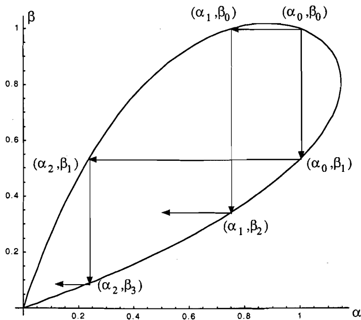
Figure 6: Curve (4.5) for \mu_1 = 2, \mu_2 = 3 and p_1 = 0.8, p_2 = 0.5
