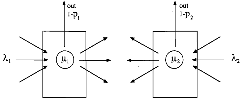
Figure 3: Standard Jackson network nodes
